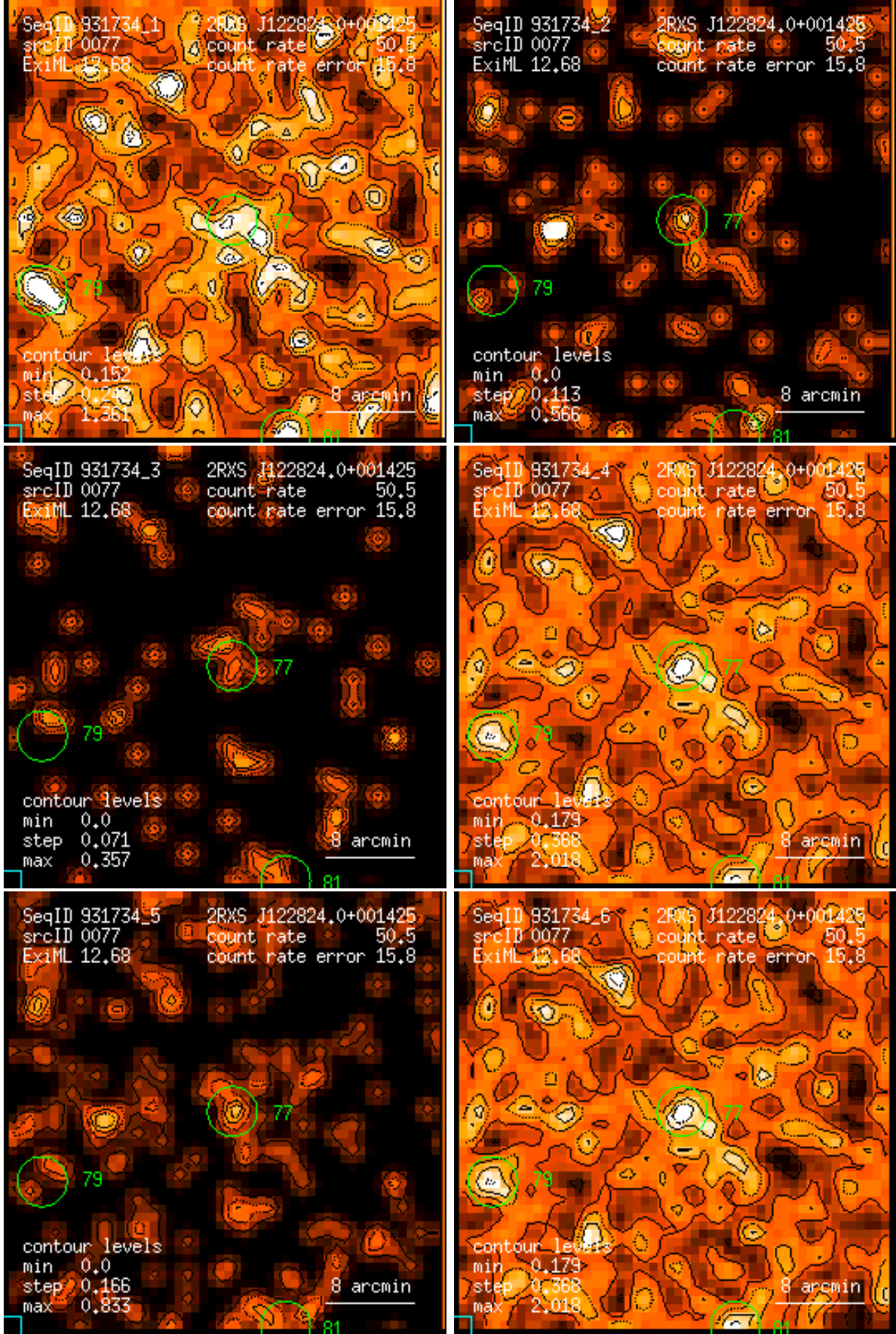
Figure 77: RASS 931734: detection 0077: band rate images, Gaussian filter: (1) PSPC channels 11 – 41, (2) 52 – 90, (3) 91 – 201, (4) 11 – 235, (5) 52 – 201, (6) 11 – 201. Broad band rates in counts/ks. Band rate contour levels in counts/ks/arcmin 2 .
