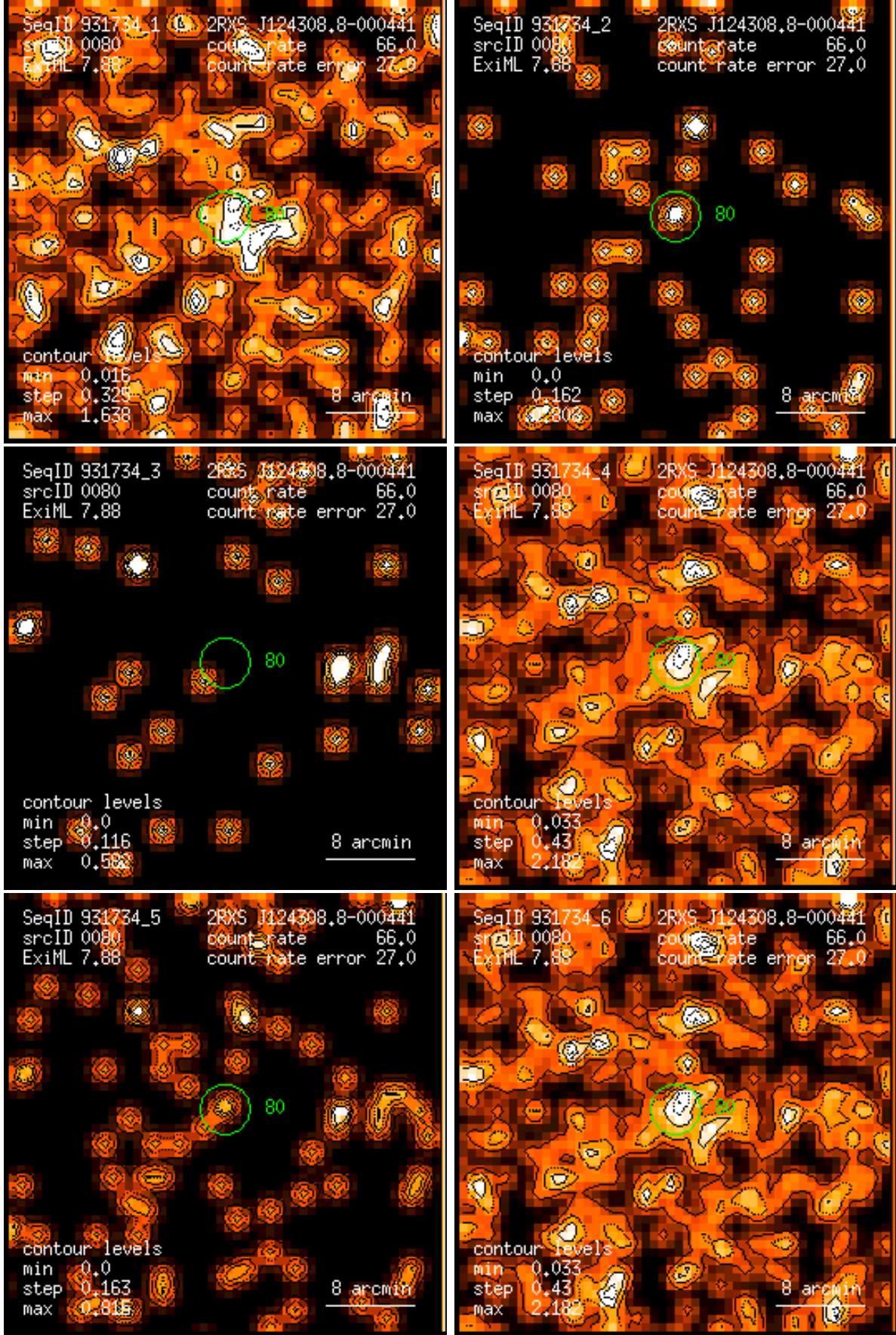
Figure 80: RASS 931734: detection 0080: band rate images, Gaussian filter: (1) PSPC channels 11 – 41, (2) 52 – 90, (3) 91 – 201, (4) 11 – 235, (5) 52 – 201, (6) 11 – 201. Broad band rates in counts/ks. Band rate contour levels in counts/ks/arcmin 2 .
