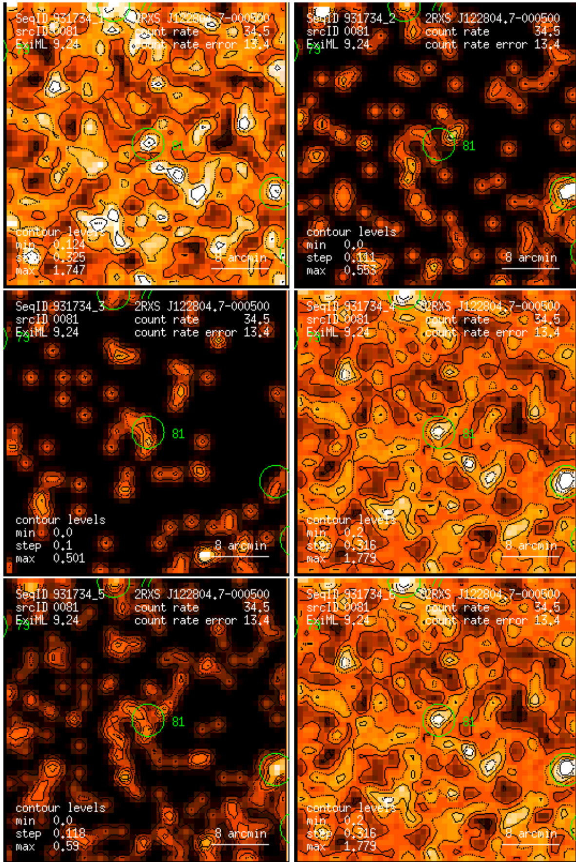
Figure 81: RASS 931734: detection 0081: band rate images, Gaussian filter: (1) PSPC channels 11 – 41, (2) 52 – 90, (3) 91 – 201, (4) 11 – 235, (5) 52 – 201, (6) 11 – 201. Broad band rates in counts/ks. Band rate contour levels in counts/ks/arcmin 2 .
