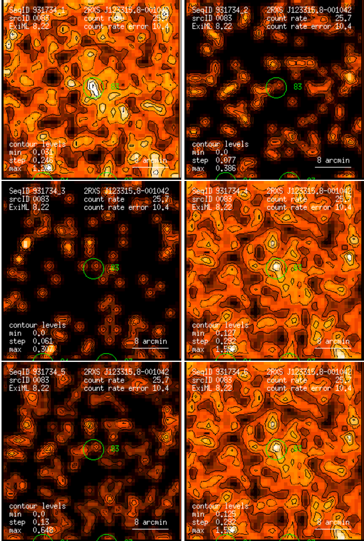
Figure 83: RASS 931734: detection 0083: band rate images, Gaussian filter: (1) PSPC channels 11 – 41, (2) 52 – 90, (3) 91 – 201, (4) 11 – 235, (5) 52 – 201, (6) 11 – 201. Broad band rates in counts/ks. Band rate contour levels in counts/ks/arcmin 2 .
