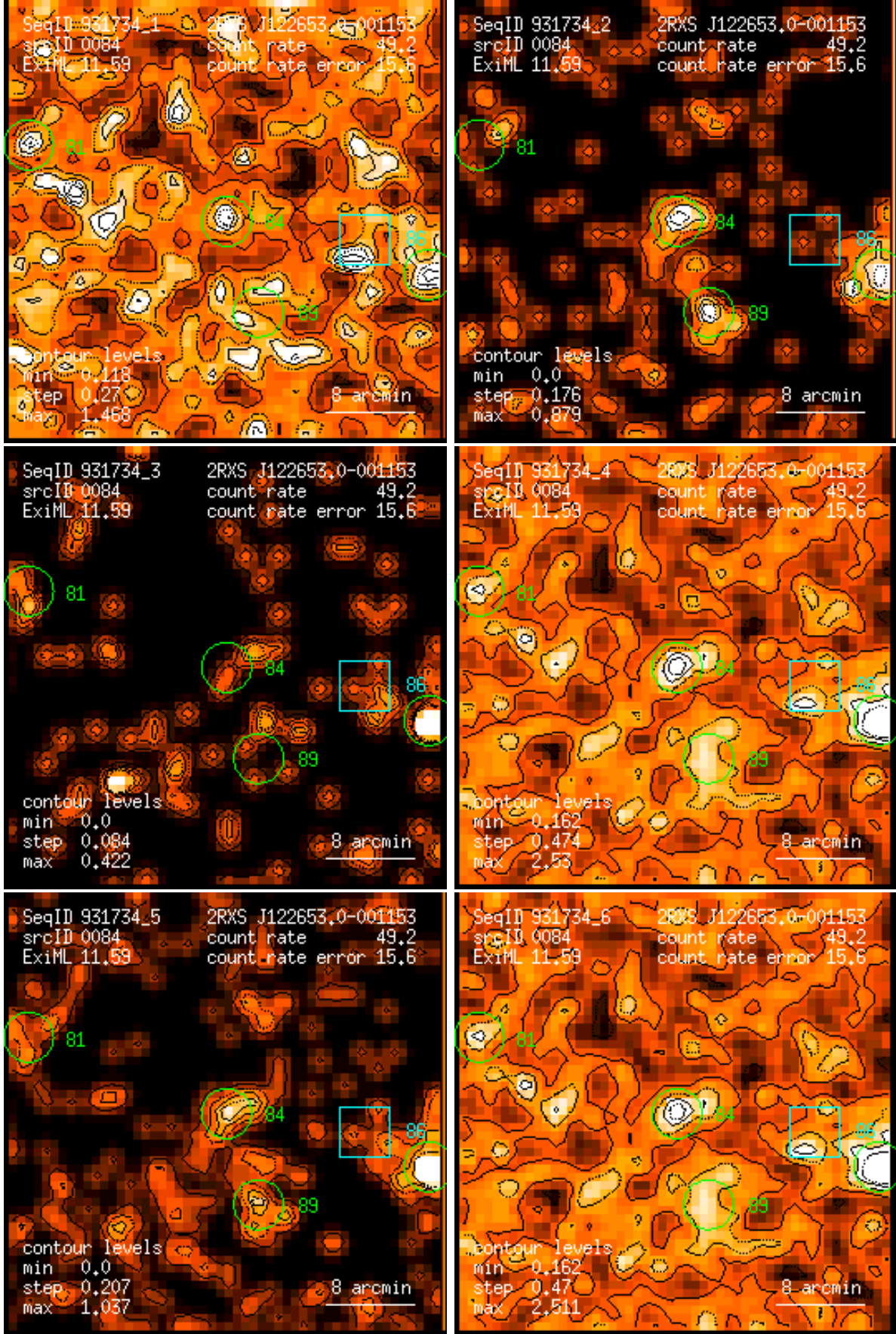
Figure 84: RASS 931734: detection 0084: band rate images, Gaussian filter: (1) PSPC channels 11 – 41, (2) 52 – 90, (3) 91 – 201, (4) 11 – 235, (5) 52 – 201, (6) 11 – 201. Broad band rates in counts/ks. Band rate contour levels in counts/ks/arcmin 2 .
