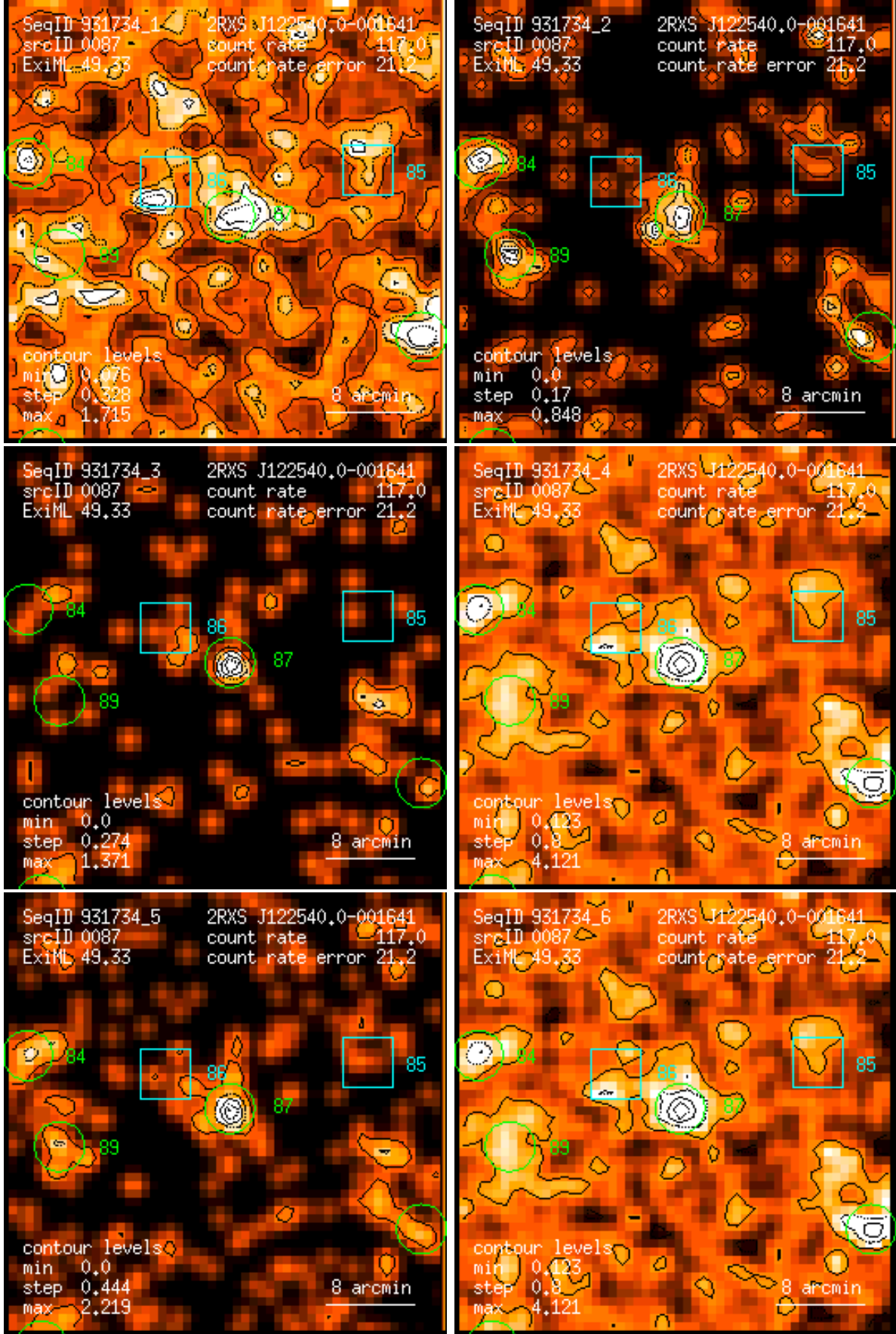
Figure 87: RASS 931734: detection 0087: band rate images, Gaussian filter: (1) PSPC channels 11 – 41, (2) 52 – 90, (3) 91 – 201, (4) 11 – 235, (5) 52 – 201, (6) 11 – 201. Broad band rates in counts/ks. Band rate contour levels in counts/ks/arcmin 2 .
