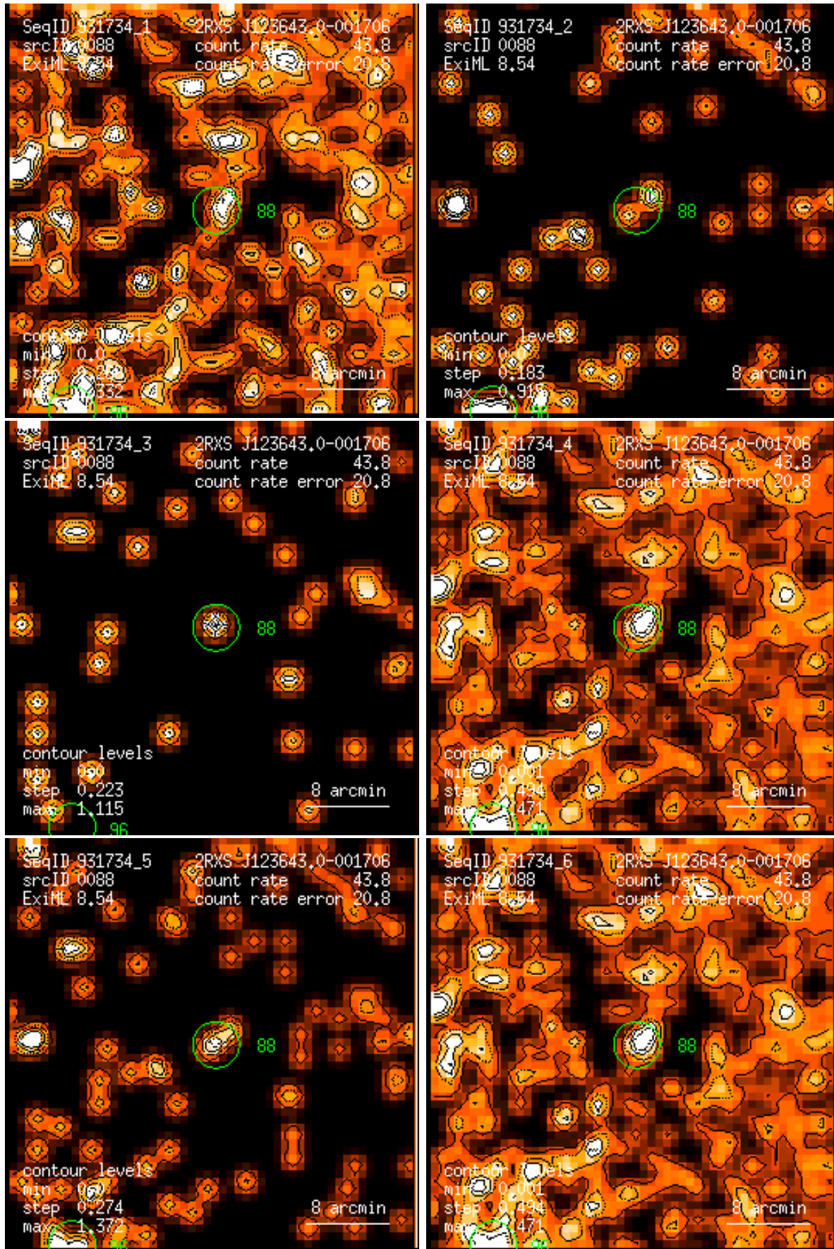
Figure 88: RASS 931734: detection 0088: band rate images, Gaussian filter: (1) PSPC channels 11 – 41, (2) 52 – 90, (3) 91 – 201, (4) 11 – 235, (5) 52 – 201, (6) 11 – 201. Broad band rates in counts/ks. Band rate contour levels in counts/ks/arcmin 2 .
