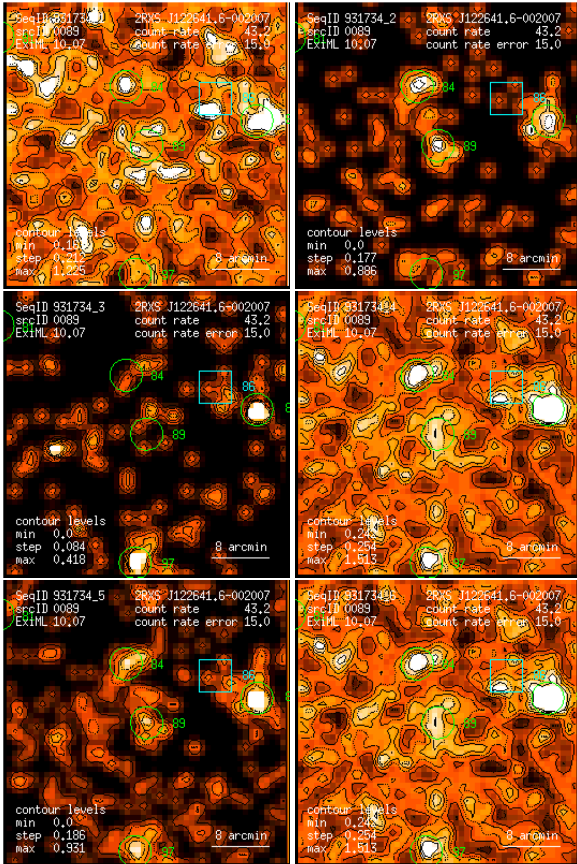
Figure 89: RASS 931734: detection 0089: band rate images, Gaussian filter: (1) PSPC channels 11 – 41, (2) 52 – 90, (3) 91 – 201, (4) 11 – 235, (5) 52 – 201, (6) 11 – 201. Broad band rates in counts/ks. Band rate contour levels in counts/ks/arcmin 2 .
