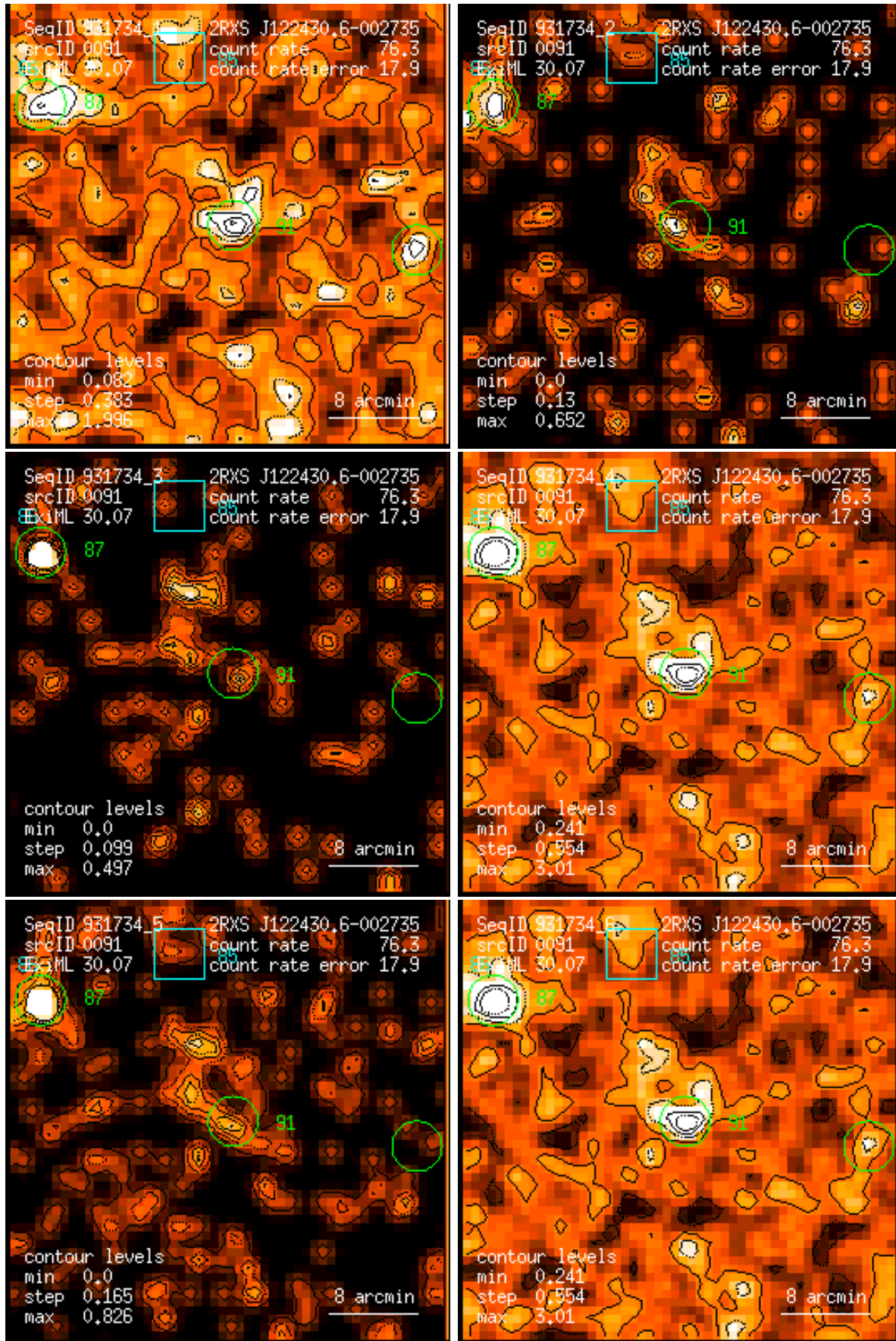
Figure 91: RASS 931734: detection 0091: band rate images, Gaussian filter: (1) PSPC channels 11 – 41, (2) 52 – 90, (3) 91 – 201, (4) 11 – 235, (5) 52 – 201, (6) 11 – 201. Broad band rates in counts/ks. Band rate contour levels in counts/ks/arcmin 2 .
