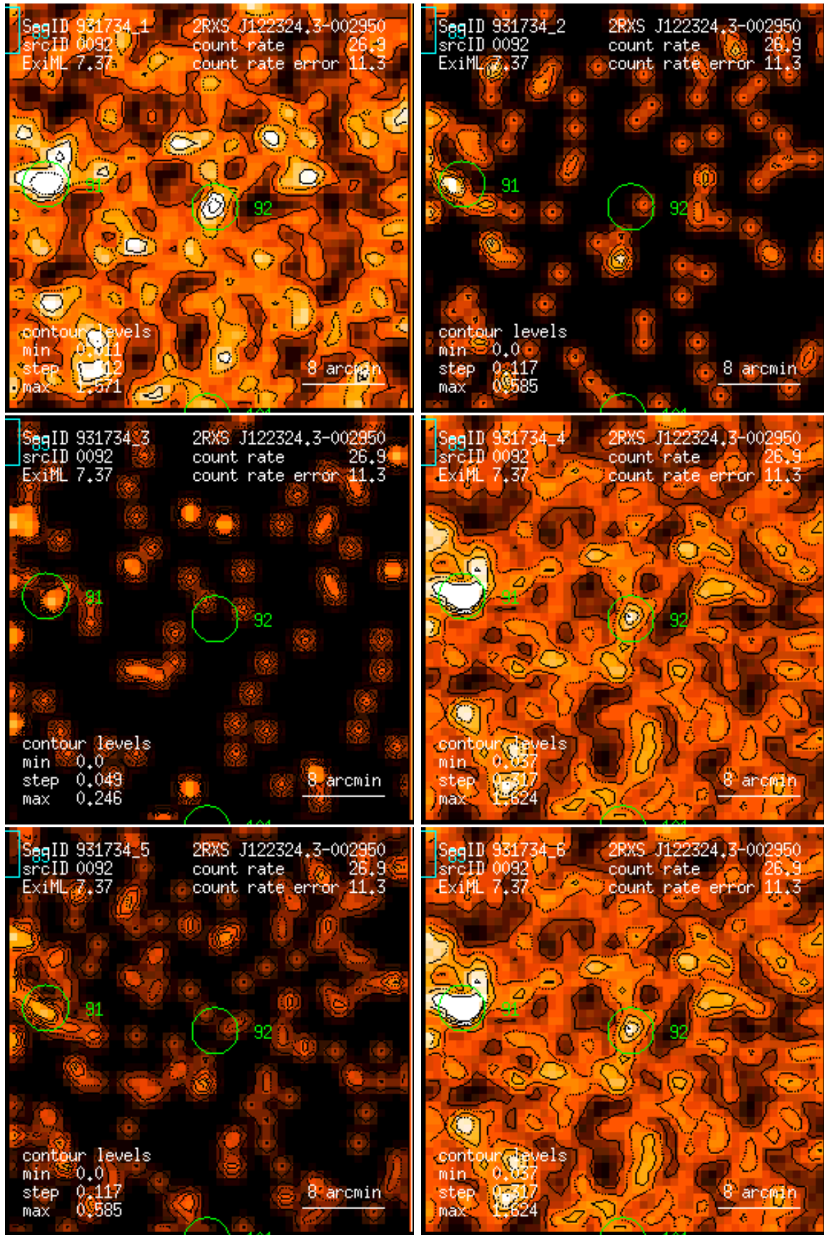
Figure 92: RASS 931734: detection 0092: band rate images, Gaussian filter: (1) PSPC channels 11 – 41, (2) 52 – 90, (3) 91 – 201, (4) 11 – 235, (5) 52 – 201, (6) 11 – 201. Broad band rates in counts/ks. Band rate contour levels in counts/ks/arcmin 2 .
