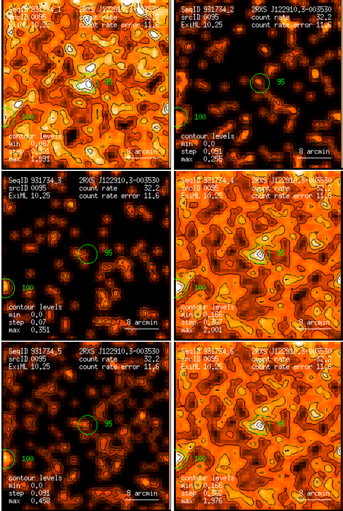
Figure 95: RASS 931734: detection 0095: band rate images, Gaussian filter: (1) PSPC channels 11 – 41, (2) 52 – 90, (3) 91 – 201, (4) 11 – 235, (5) 52 – 201, (6) 11 – 201. Broad band rates in counts/ks. Band rate contour levels in counts/ks/arcmin 2 .
