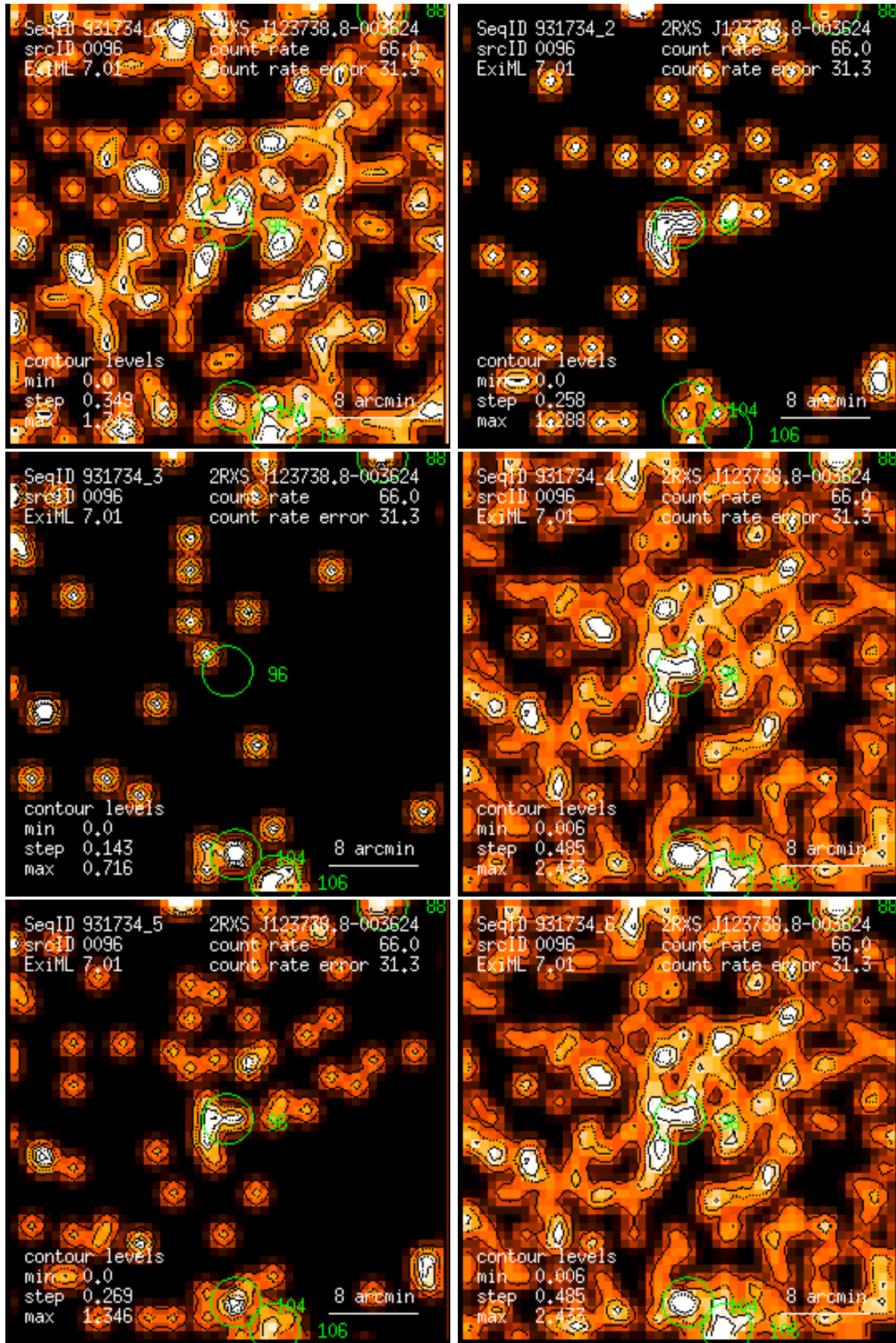
Figure 96: RASS 931734: detection 0096: band rate images, Gaussian filter: (1) PSPC channels 11 – 41, (2) 52 – 90, (3) 91 – 201, (4) 11 – 235, (5) 52 – 201, (6) 11 – 201. Broad band rates in counts/ks. Band rate contour levels in counts/ks/arcmin 2 .
