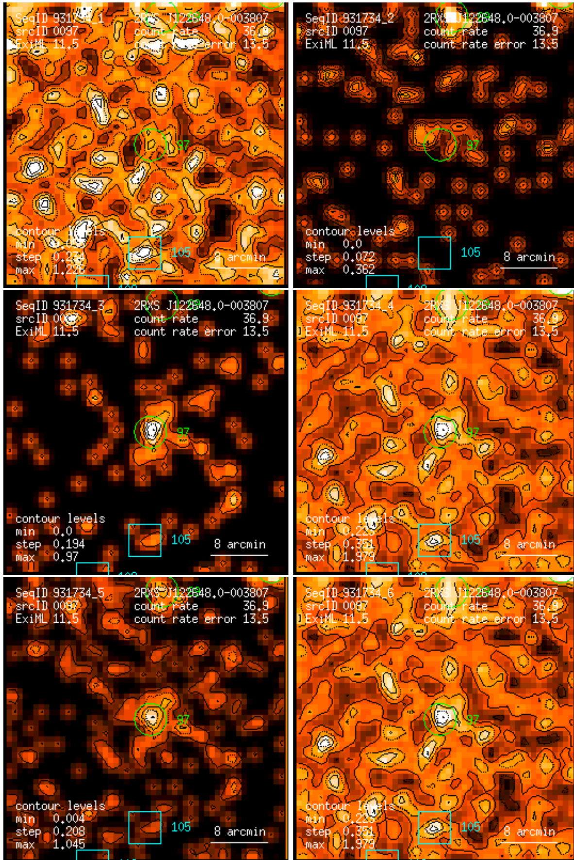
Figure 97: RASS 931734: detection 0097: band rate images, Gaussian filter: (1) PSPC channels 11 – 41, (2) 52 – 90, (3) 91 – 201, (4) 11 – 235, (5) 52 – 201, (6) 11 – 201. Broad band rates in counts/ks. Band rate contour levels in counts/ks/arcmin 2 .
