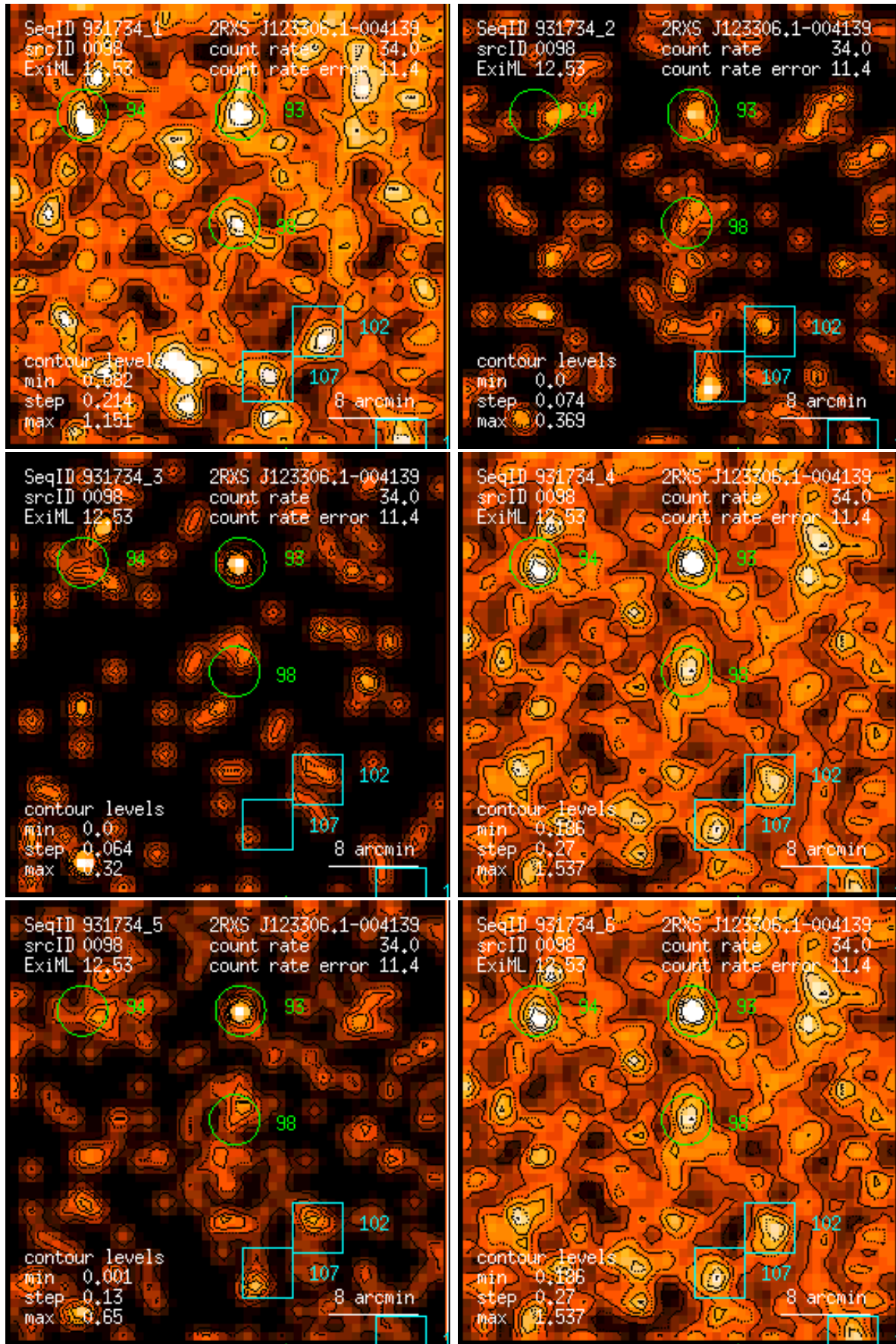
Figure 98: RASS 931734: detection 0098: band rate images, Gaussian filter: (1) PSPC channels 11 – 41, (2) 52 – 90, (3) 91 – 201, (4) 11 – 235, (5) 52 – 201, (6) 11 – 201. Broad band rates in counts/ks. Band rate contour levels in counts/ks/arcmin 2 .
