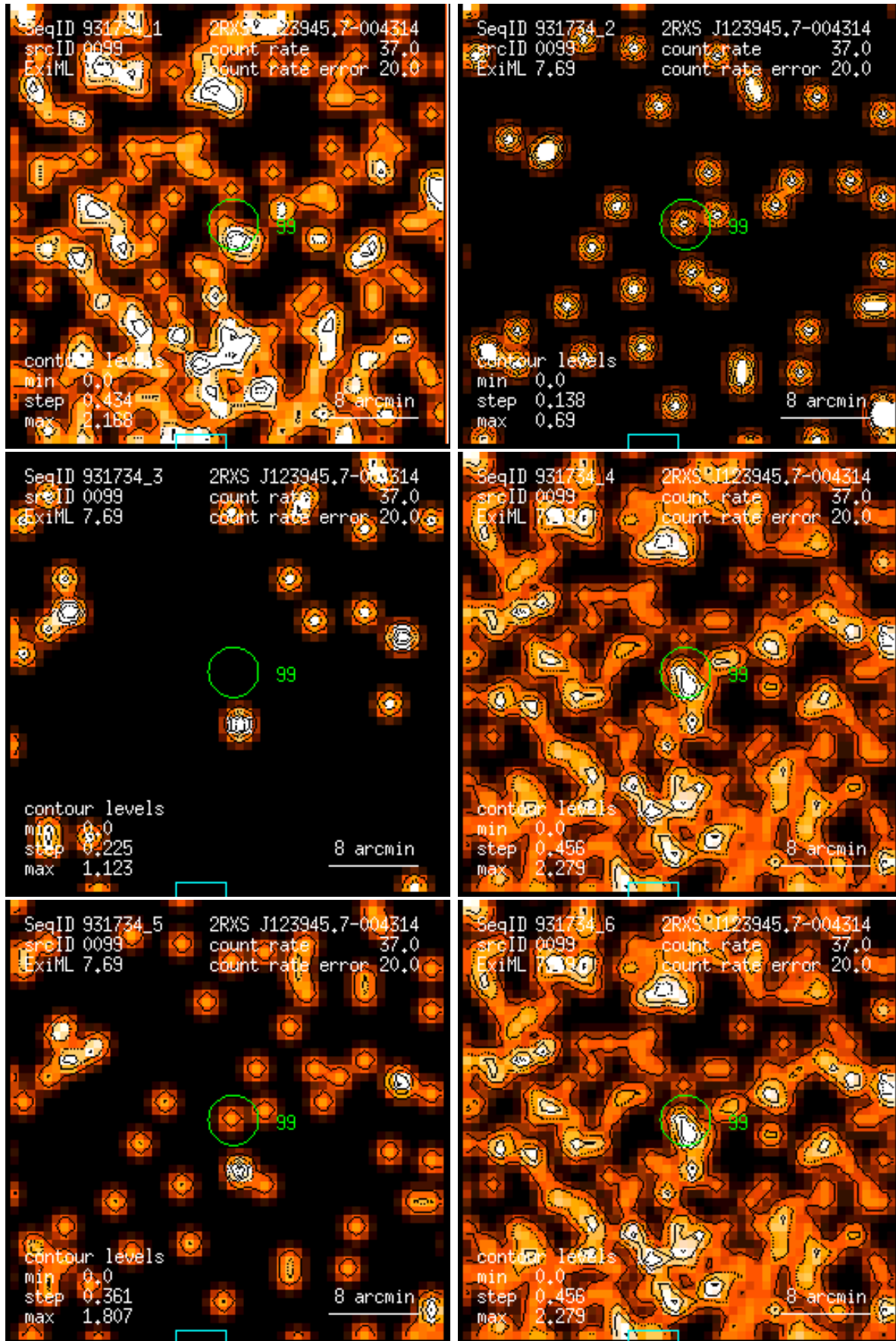
Figure 99: RASS 931734: detection 0099: band rate images, Gaussian filter: (1) PSPC channels 11 – 41, (2) 52 – 90, (3) 91 – 201, (4) 11 – 235, (5) 52 – 201, (6) 11 – 201. Broad band rates in counts/ks. Band rate contour levels in counts/ks/arcmin 2 .
