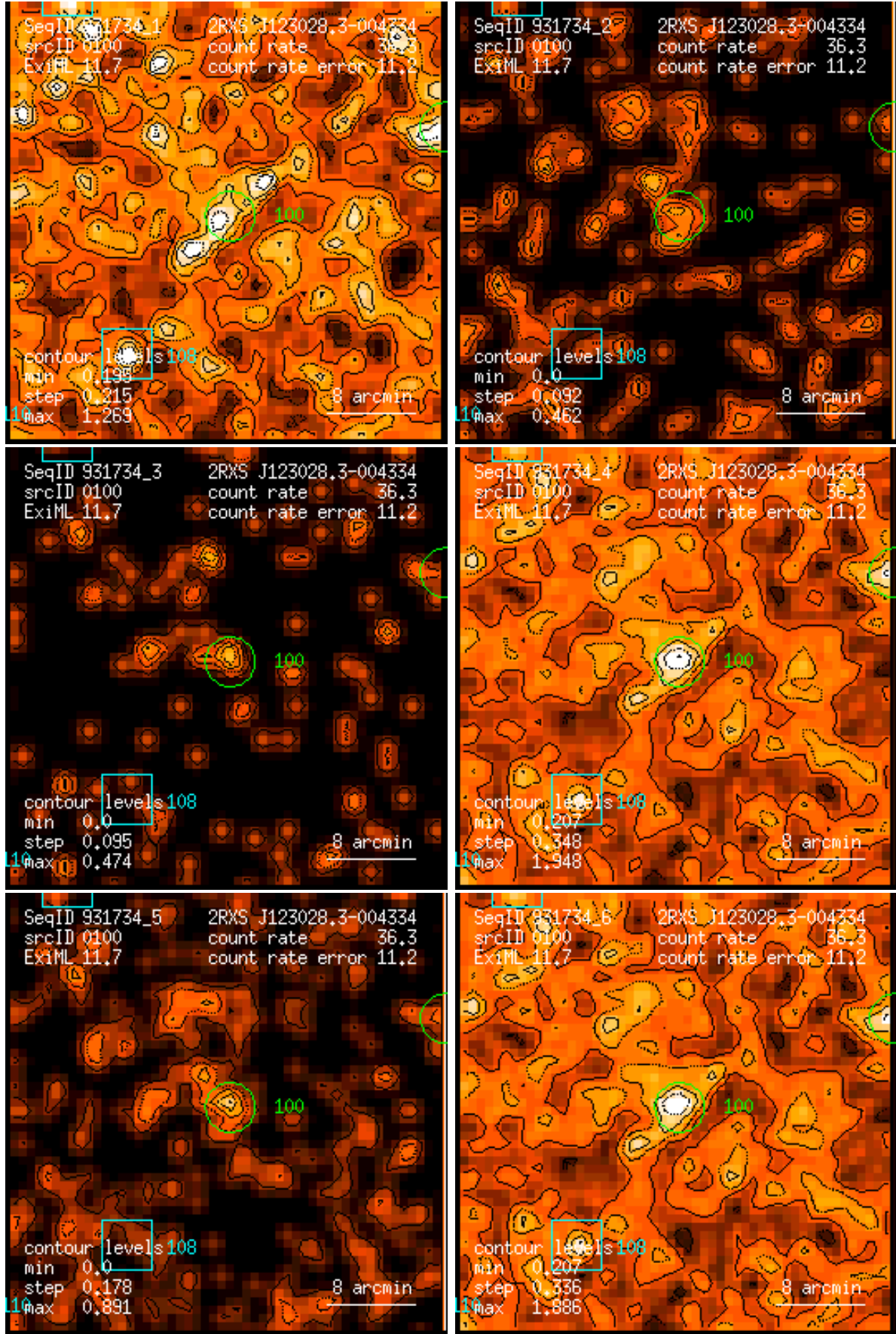
Figure 100: RASS 931734: detection 0100: band rate images, Gaussian filter: (1) PSPC channels 11 – 41, (2) 52 – 90, (3) 91 – 201, (4) 11 – 235, (5) 52 – 201, (6) 11 – 201. Broad band rates in counts/ks. Band rate contour levels in counts/ks/arcmin 2 .
