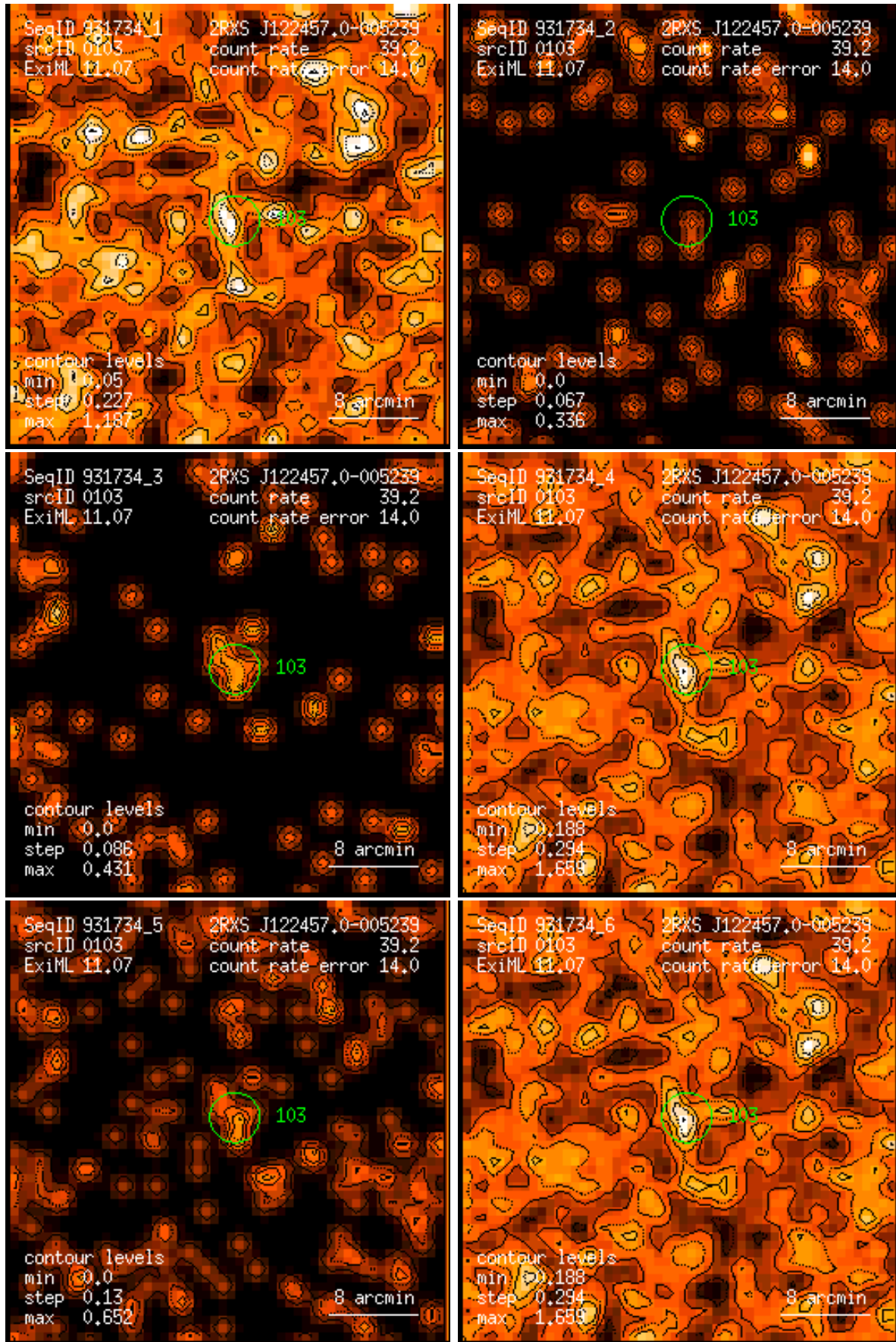
Figure 103: RASS 931734: detection 0103: band rate images, Gaussian filter: (1) PSPC channels 11 – 41, (2) 52 – 90, (3) 91 – 201, (4) 11 – 235, (5) 52 – 201, (6) 11 – 201. Broad band rates in counts/ks. Band rate contour levels in counts/ks/arcmin 2 .
