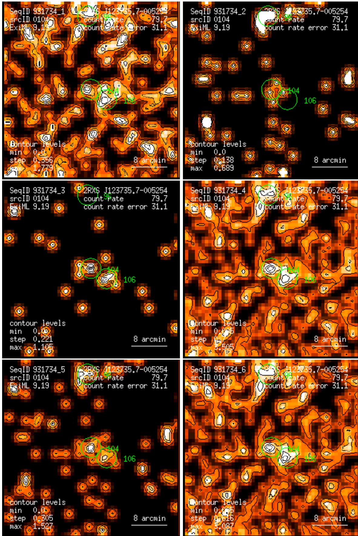
Figure 104: RASS 931734: detection 0104: band rate images, Gaussian filter: (1) PSPC channels 11 – 41, (2) 52 – 90, (3) 91 – 201, (4) 11 – 235, (5) 52 – 201, (6) 11 – 201. Broad band rates in counts/ks. Band rate contour levels in counts/ks/arcmin 2 .
