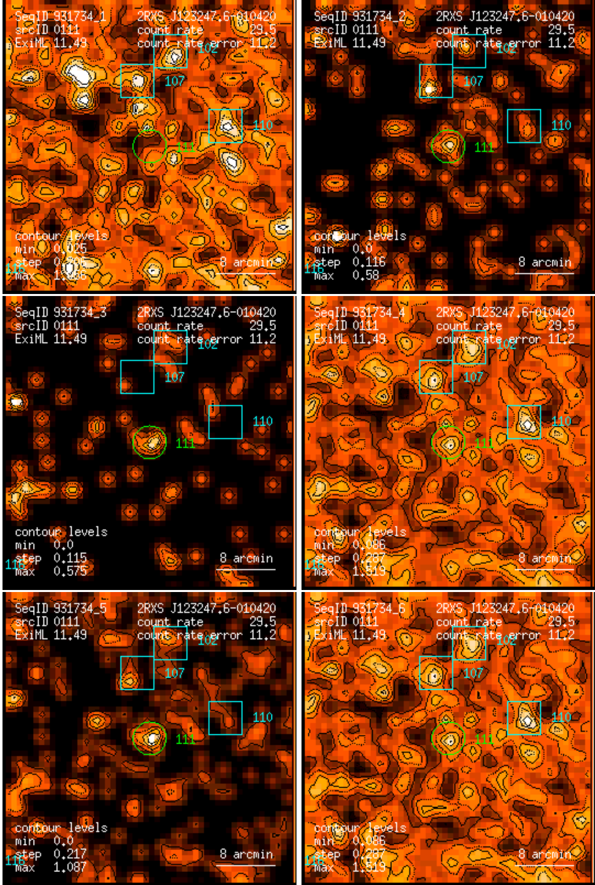
Figure 111: RASS 931734: detection 0111: band rate images, Gaussian filter: (1) PSPC channels 11 – 41, (2) 52 – 90, (3) 91 – 201, (4) 11 – 235, (5) 52 – 201, (6) 11 – 201. Broad band rates in counts/ks. Band rate contour levels in counts/ks/arcmin 2 .
