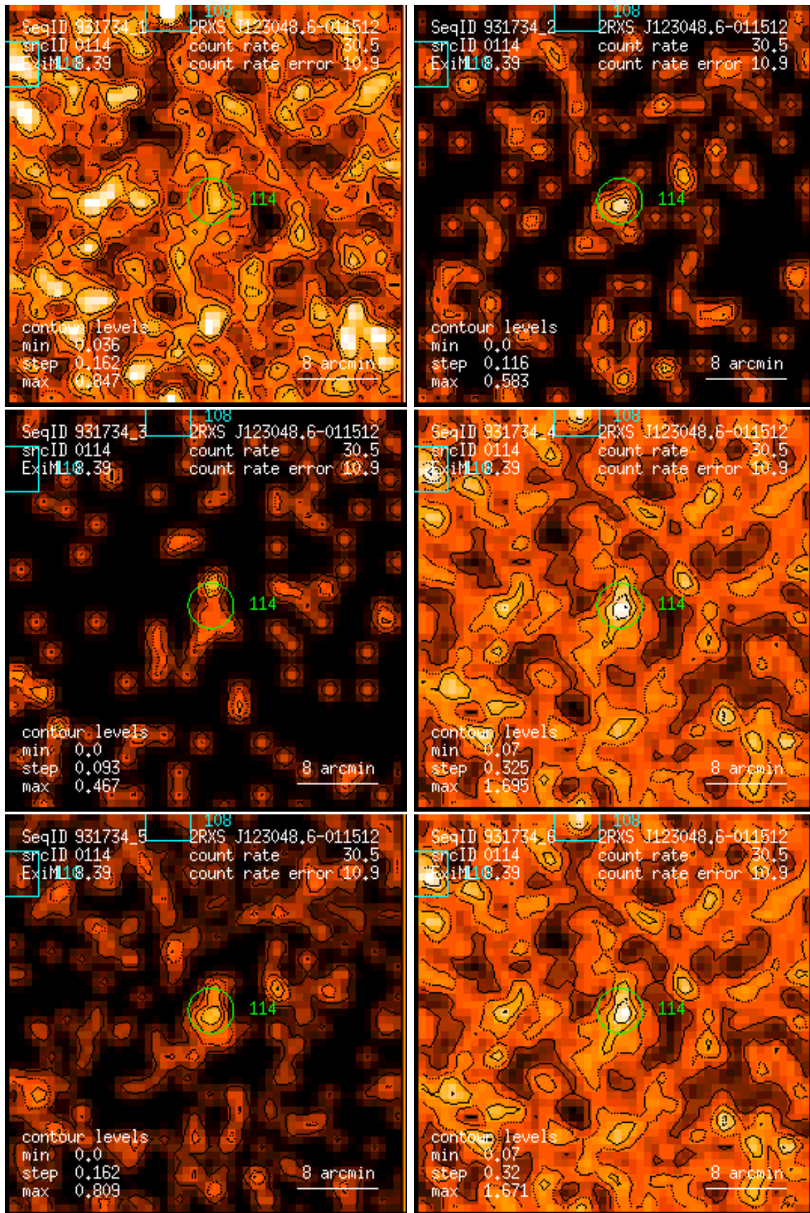
Figure 114: RASS 931734: detection 0114: band rate images, Gaussian filter: (1) PSPC channels 11 – 41, (2) 52 – 90, (3) 91 – 201, (4) 11 – 235, (5) 52 – 201, (6) 11 – 201. Broad band rates in counts/ks. Band rate contour levels in counts/ks/arcmin 2 .
