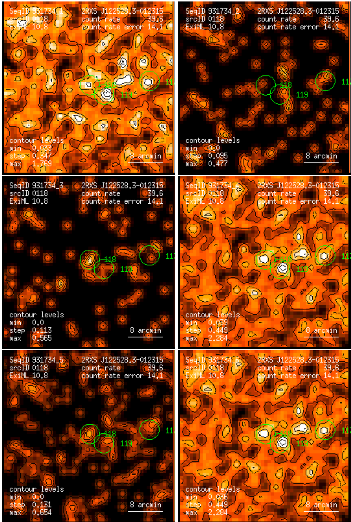
Figure 118: RASS 931734: detection 0118: band rate images, Gaussian filter: (1) PSPC channels 11 – 41, (2) 52 – 90, (3) 91 – 201, (4) 11 – 235, (5) 52 – 201, (6) 11 – 201. Broad band rates in counts/ks. Band rate contour levels in counts/ks/arcmin 2 .
