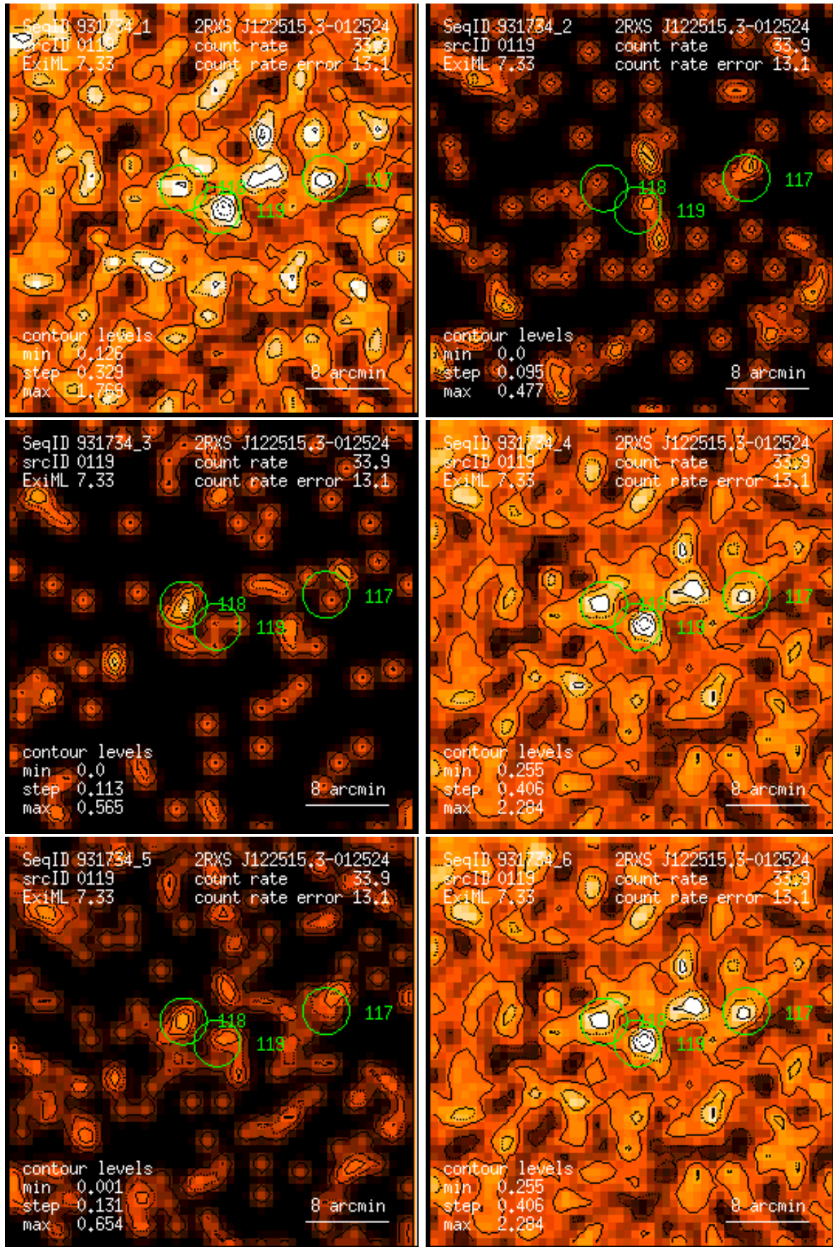
Figure 119: RASS 931734: detection 0119: band rate images, Gaussian filter: (1) PSPC channels 11 – 41, (2) 52 – 90, (3) 91 – 201, (4) 11 – 235, (5) 52 – 201, (6) 11 – 201. Broad band rates in counts/ks. Band rate contour levels in counts/ks/arcmin 2 .
