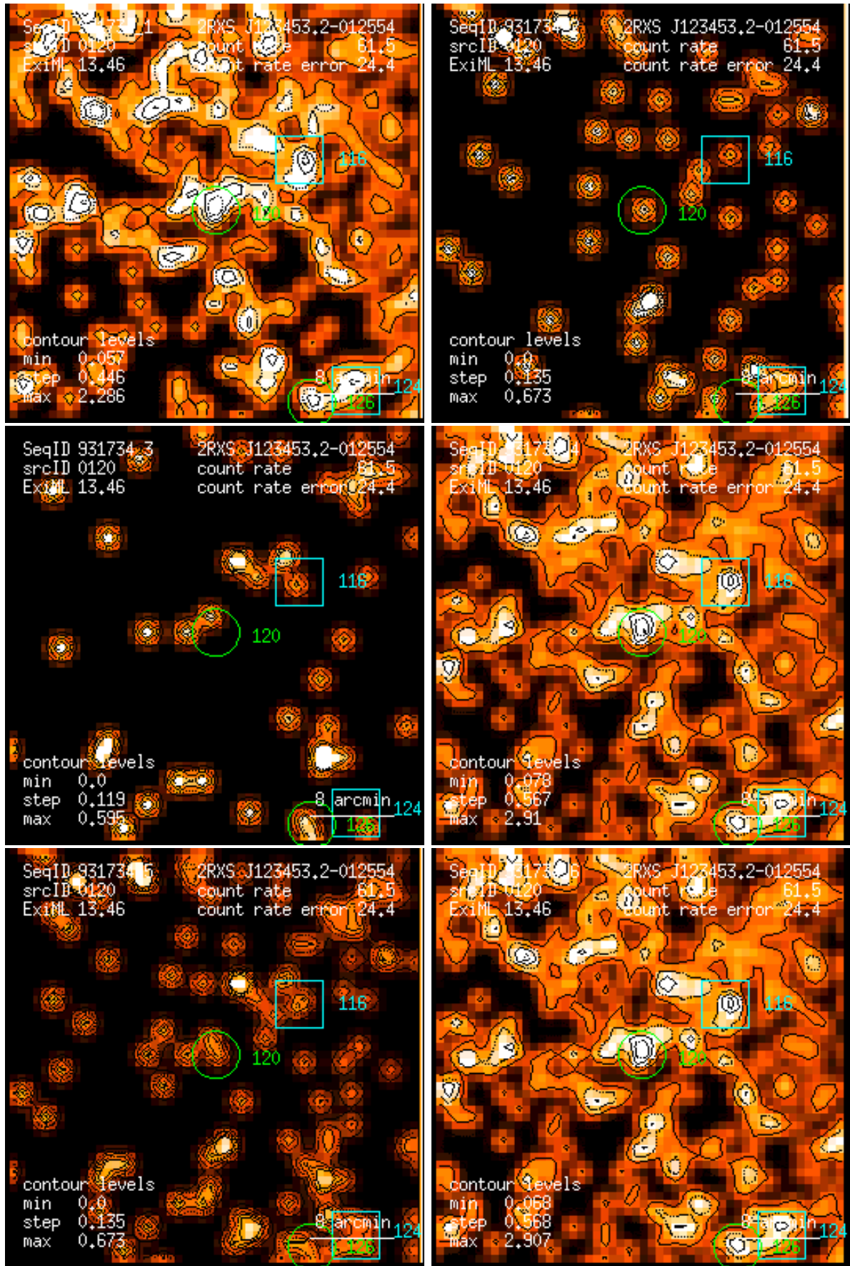
Figure 120: RASS 931734: detection 0120: band rate images, Gaussian filter: (1) PSPC channels 11 – 41, (2) 52 – 90, (3) 91 – 201, (4) 11 – 235, (5) 52 – 201, (6) 11 – 201. Broad band rates in counts/ks. Band rate contour levels in counts/ks/arcmin 2 .
