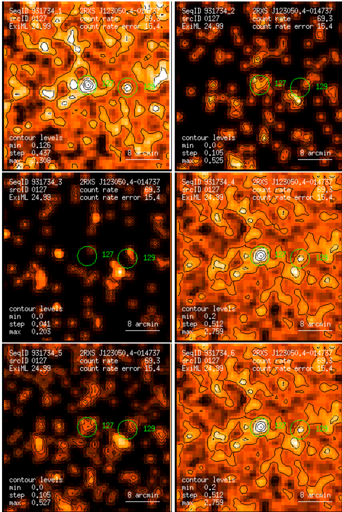
Figure 127: RASS 931734: detection 0127: band rate images, Gaussian filter: (1) PSPC channels 11 – 41, (2) 52 – 90, (3) 91 – 201, (4) 11 – 235, (5) 52 – 201, (6) 11 – 201. Broad band rates in counts/ks. Band rate contour levels in counts/ks/arcmin 2 .
