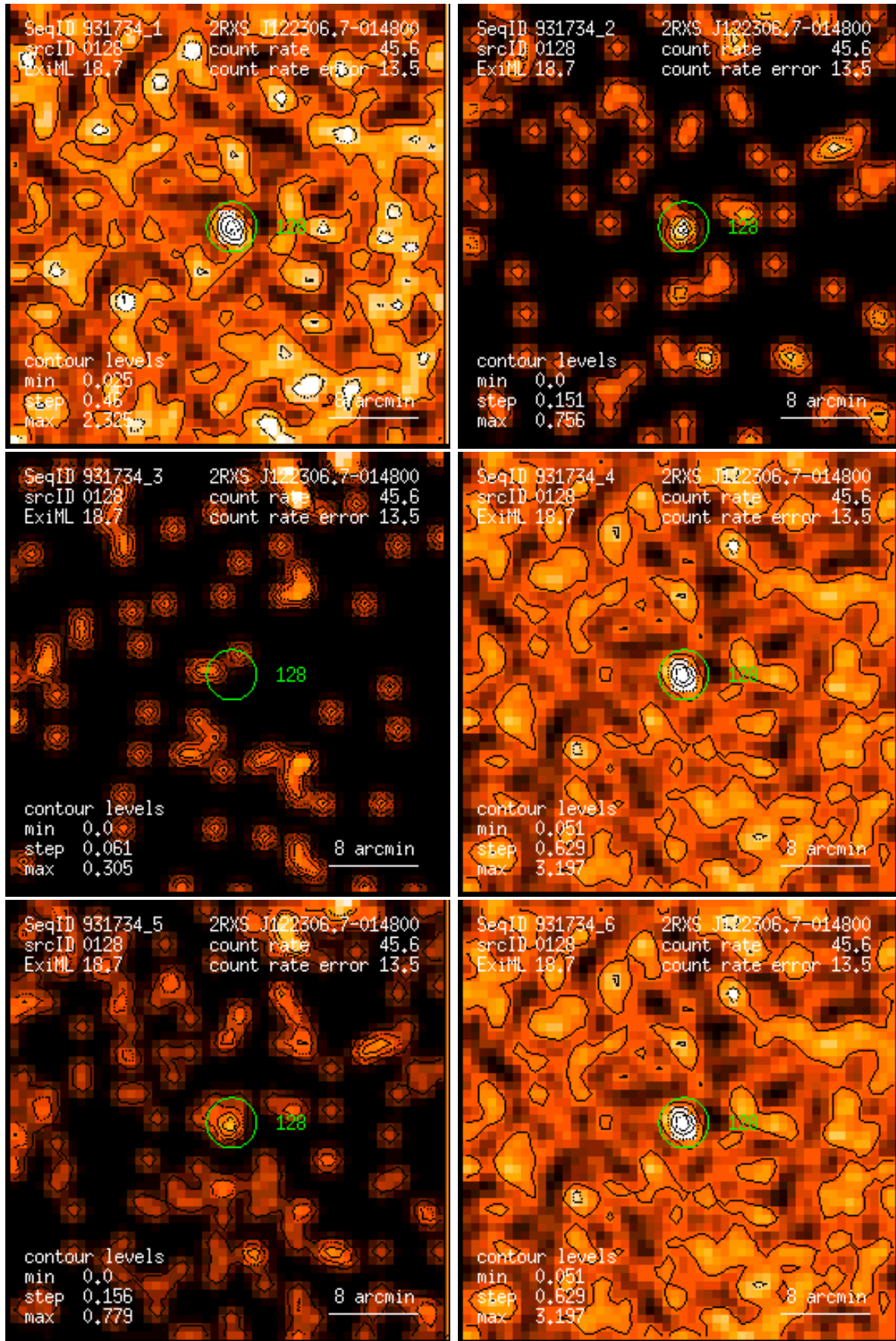
Figure 128: RASS 931734: detection 0128: band rate images, Gaussian filter: (1) PSPC channels 11 – 41, (2) 52 – 90, (3) 91 – 201, (4) 11 – 235, (5) 52 – 201, (6) 11 – 201. Broad band rates in counts/ks. Band rate contour levels in counts/ks/arcmin 2 .
