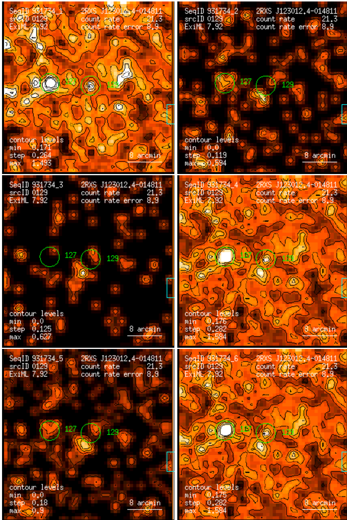
Figure 129: RASS 931734: detection 0129: band rate images, Gaussian filter: (1) PSPC channels 11 – 41, (2) 52 – 90, (3) 91 – 201, (4) 11 – 235, (5) 52 – 201, (6) 11 – 201. Broad band rates in counts/ks. Band rate contour levels in counts/ks/arcmin 2 .
