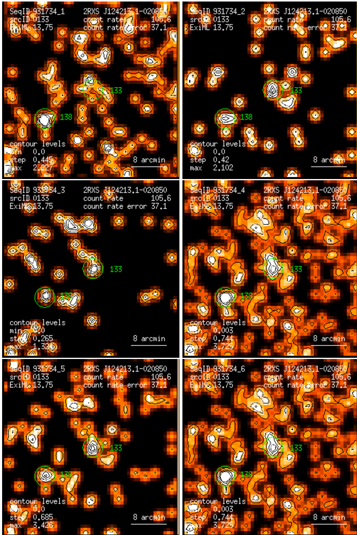
Figure 133: RASS 931734: detection 0133: band rate images, Gaussian filter: (1) PSPC channels 11 – 41, (2) 52 – 90, (3) 91 – 201, (4) 11 – 235, (5) 52 – 201, (6) 11 – 201. Broad band rates in counts/ks. Band rate contour levels in counts/ks/arcmin 2 .
