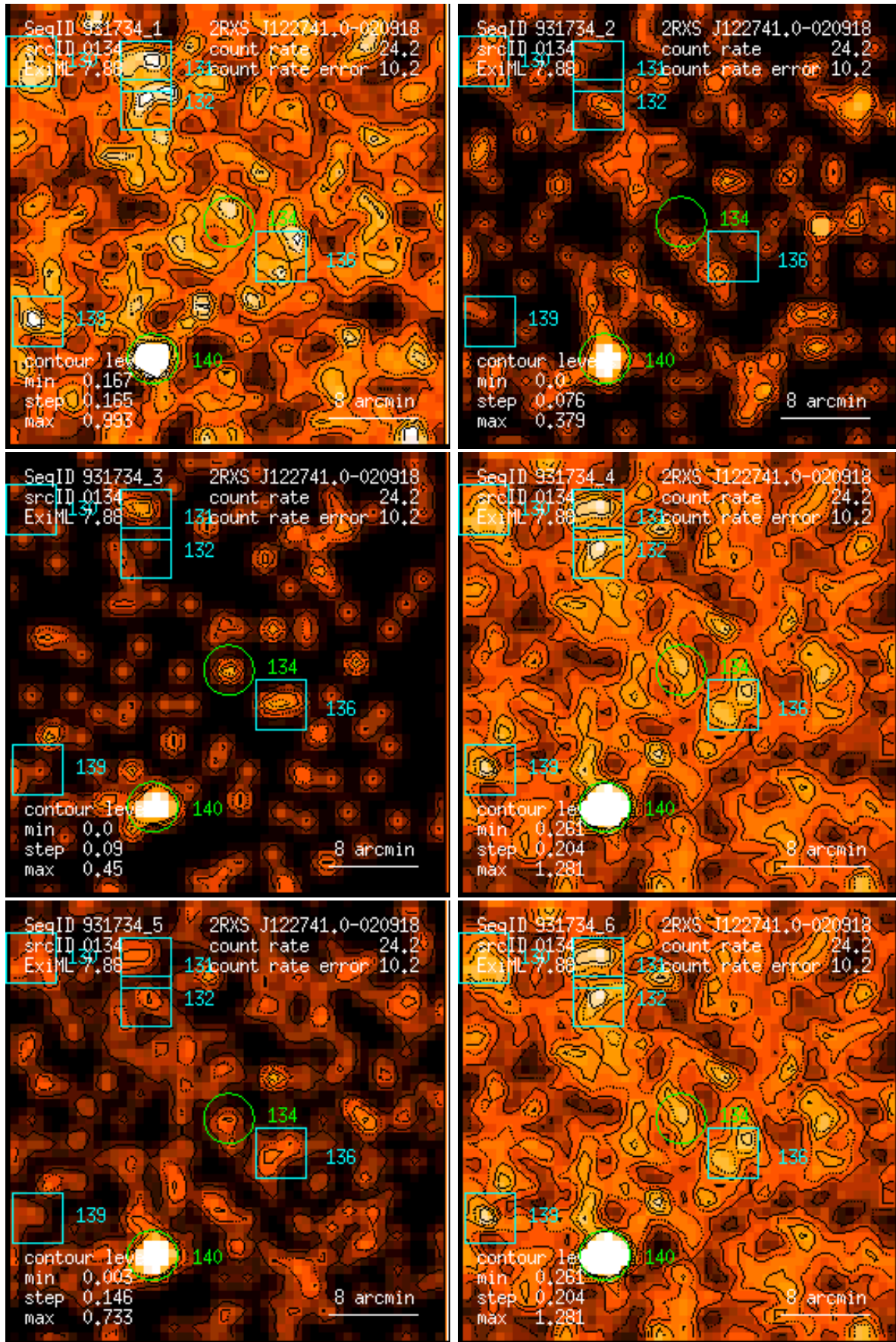
Figure 134: RASS 931734: detection 0134: band rate images, Gaussian filter: (1) PSPC channels 11 – 41, (2) 52 – 90, (3) 91 – 201, (4) 11 – 235, (5) 52 – 201, (6) 11 – 201. Broad band rates in counts/ks. Band rate contour levels in counts/ks/arcmin 2 .
