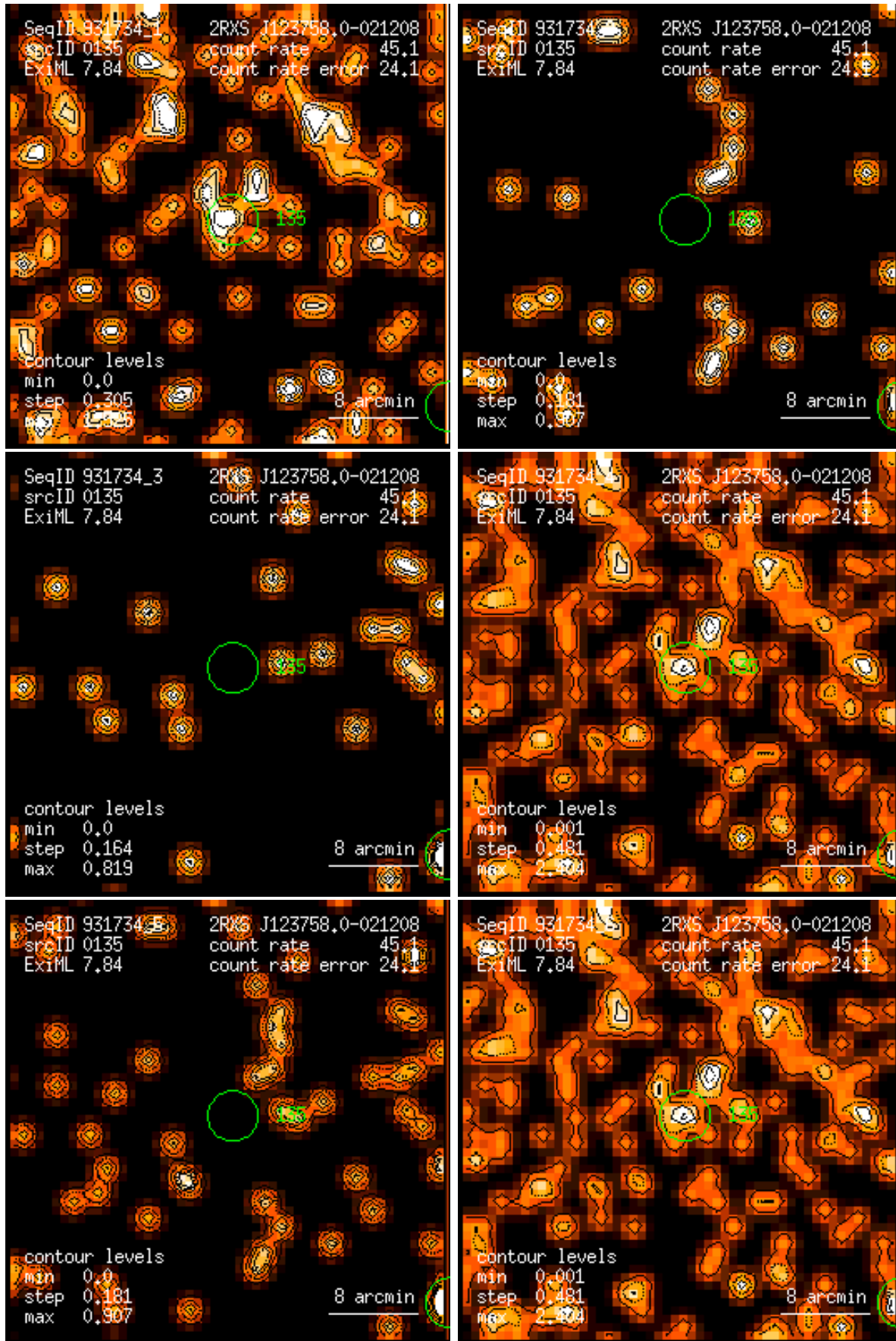
Figure 135: RASS 931734: detection 0135: band rate images, Gaussian filter: (1) PSPC channels 11 – 41, (2) 52 – 90, (3) 91 – 201, (4) 11 – 235, (5) 52 – 201, (6) 11 – 201. Broad band rates in counts/ks. Band rate contour levels in counts/ks/arcmin 2 .
