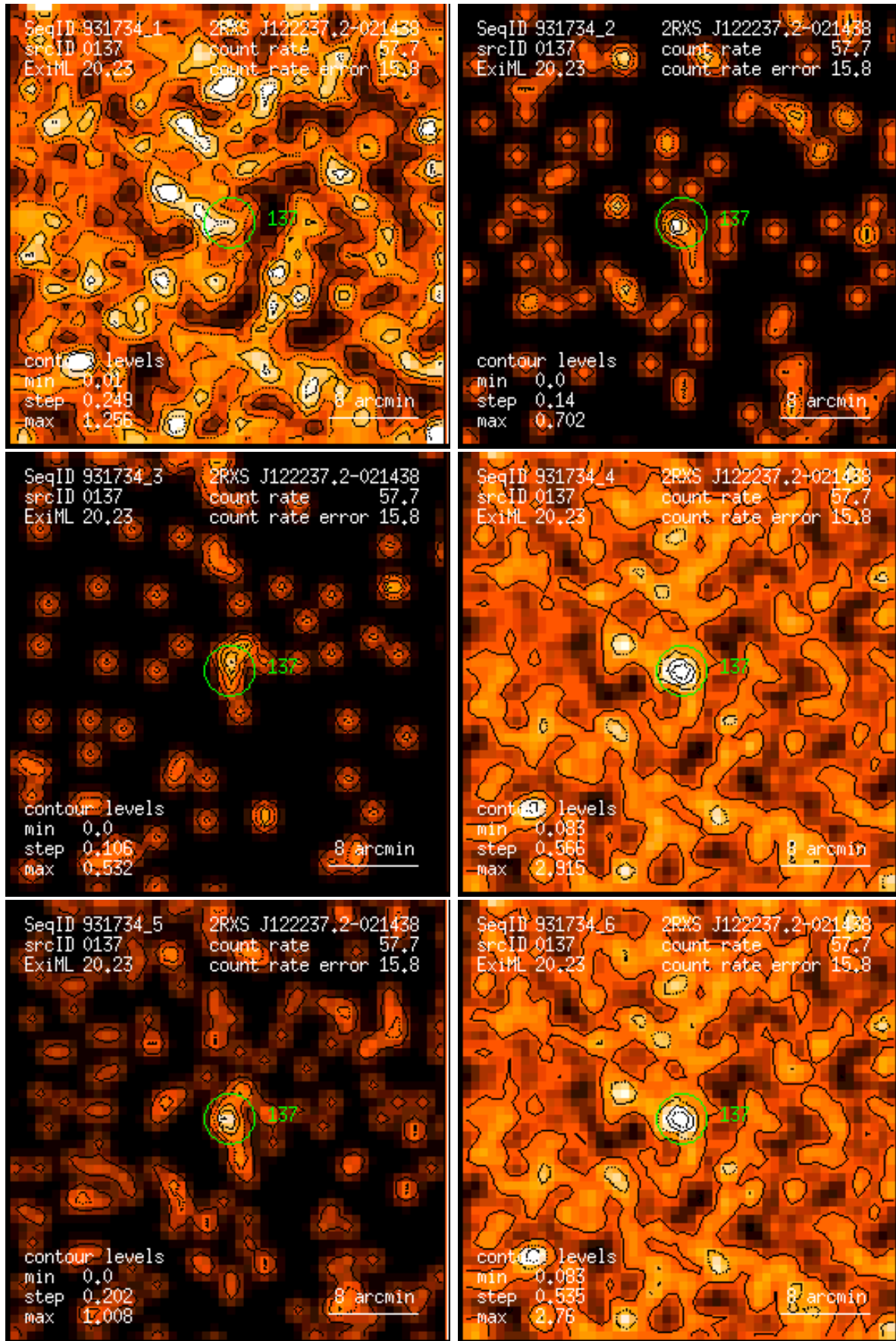
Figure 137: RASS 931734: detection 0137: band rate images, Gaussian filter: (1) PSPC channels 11 – 41, (2) 52 – 90, (3) 91 – 201, (4) 11 – 235, (5) 52 – 201, (6) 11 – 201. Broad band rates in counts/ks. Band rate contour levels in counts/ks/arcmin 2 .
