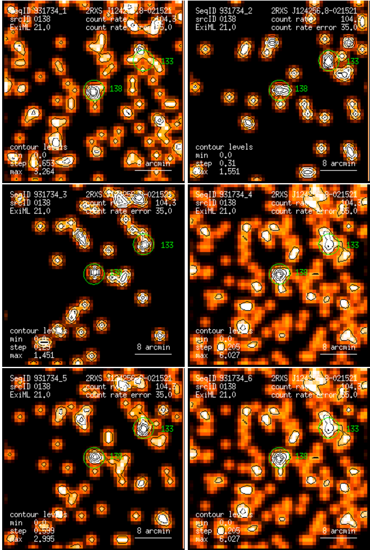
Figure 138: RASS 931734: detection 0138: band rate images, Gaussian filter: (1) PSPC channels 11 – 41, (2) 52 – 90, (3) 91 – 201, (4) 11 – 235, (5) 52 – 201, (6) 11 – 201. Broad band rates in counts/ks. Band rate contour levels in counts/ks/arcmin 2 .
