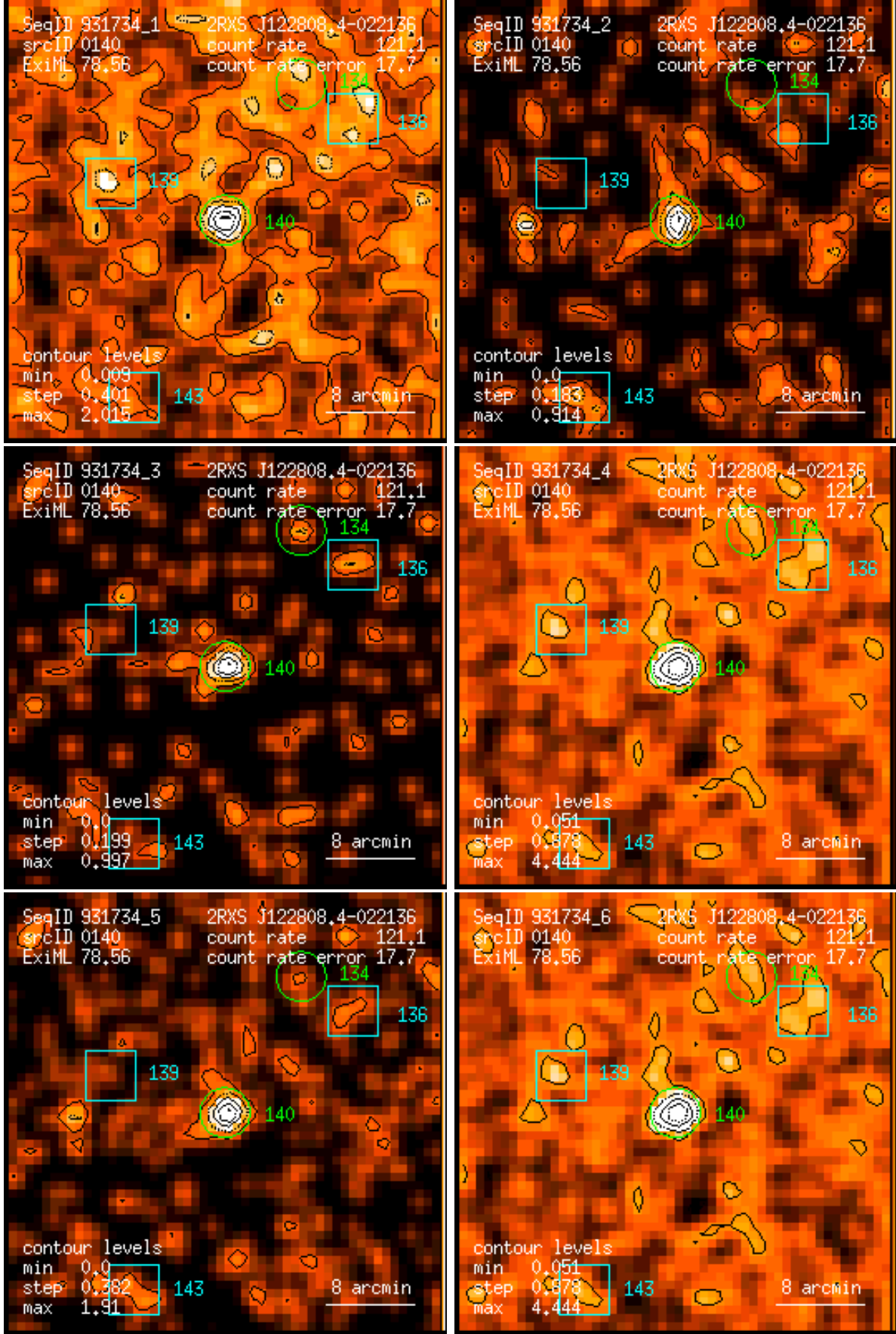
Figure 140: RASS 931734: detection 0140: band rate images, Gaussian filter: (1) PSPC channels 11 – 41, (2) 52 – 90, (3) 91 – 201, (4) 11 – 235, (5) 52 – 201, (6) 11 – 201. Broad band rates in counts/ks. Band rate contour levels in counts/ks/arcmin 2 .
