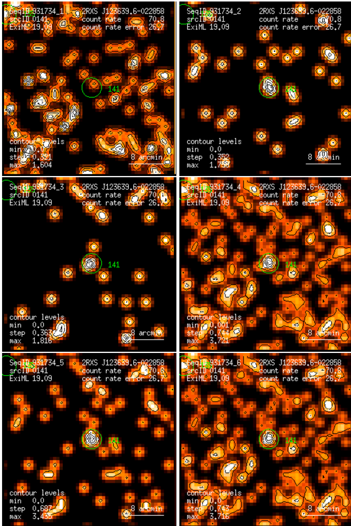
Figure 141: RASS 931734: detection 0141: band rate images, Gaussian filter: (1) PSPC channels 11 – 41, (2) 52 – 90, (3) 91 – 201, (4) 11 – 235, (5) 52 – 201, (6) 11 – 201. Broad band rates in counts/ks. Band rate contour levels in counts/ks/arcmin 2 .
