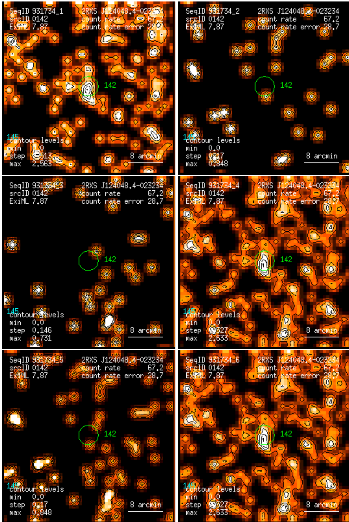
Figure 142: RASS 931734: detection 0142: band rate images, Gaussian filter: (1) PSPC channels 11 – 41, (2) 52 – 90, (3) 91 – 201, (4) 11 – 235, (5) 52 – 201, (6) 11 – 201. Broad band rates in counts/ks. Band rate contour levels in counts/ks/arcmin 2 .
