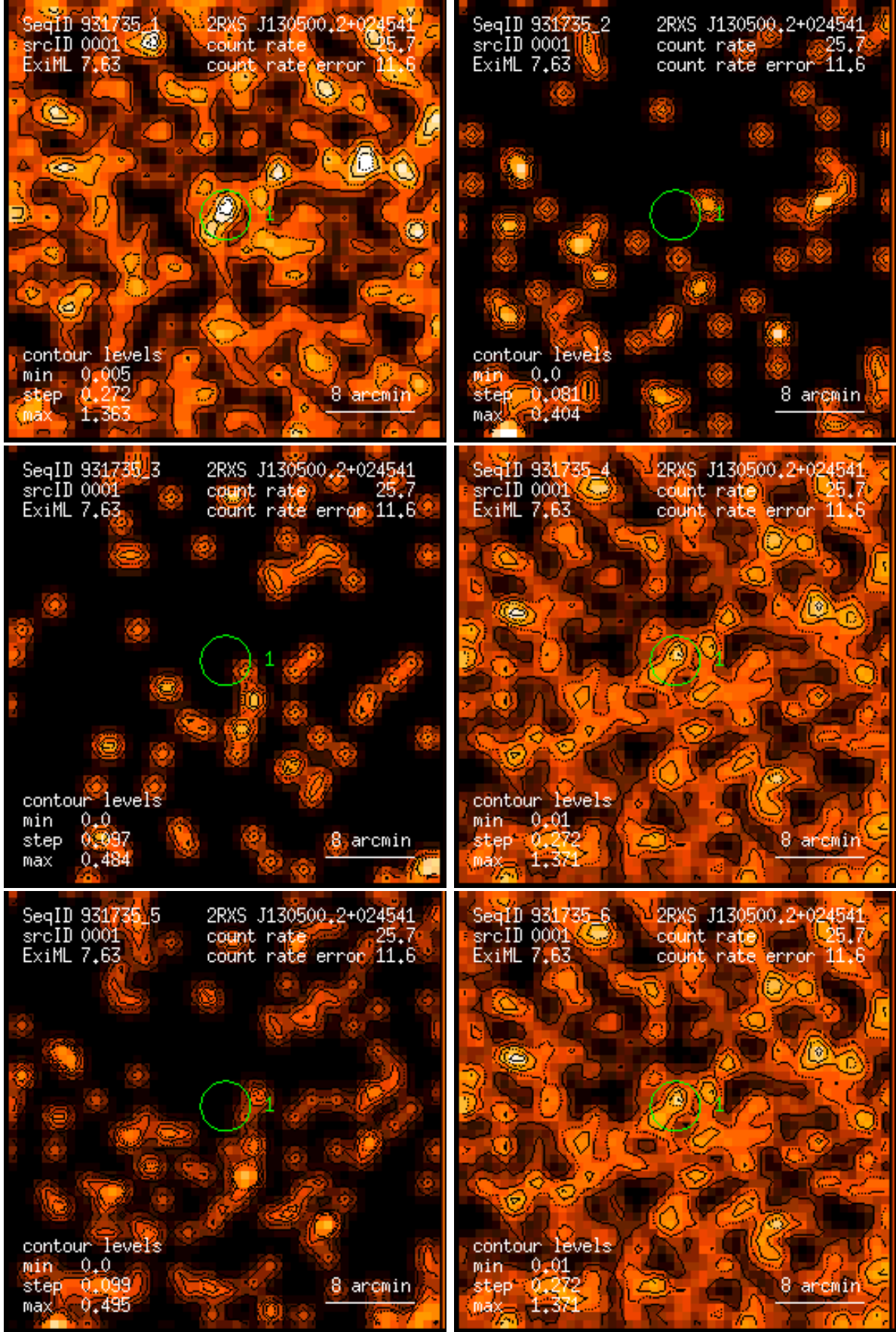
Figure 1: RASS 931735: detection 0001: band rate images, Gaussian filter: (1) PSPC channels 11 – 41, (2) 52 – 90, (3) 91 – 201, (4) 11 – 235, (5) 52 – 201, (6) 11 – 201. Broad band rates in counts/ks. Band rate contour levels in counts/ks/arcmin 2 .
