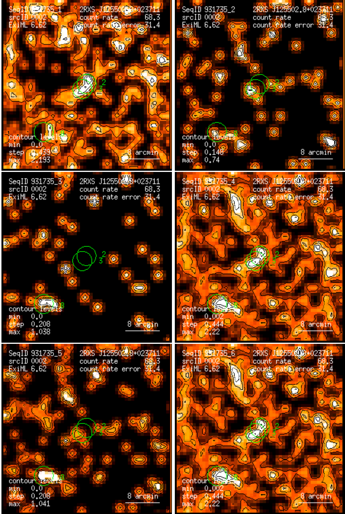
Figure 2: RASS 931735: detection 0002: band rate images, Gaussian filter: (1) PSPC channels 11 – 41, (2) 52 – 90, (3) 91 – 201, (4) 11 – 235, (5) 52 – 201, (6) 11 – 201. Broad band rates in counts/ks. Band rate contour levels in counts/ks/arcmin 2 .
