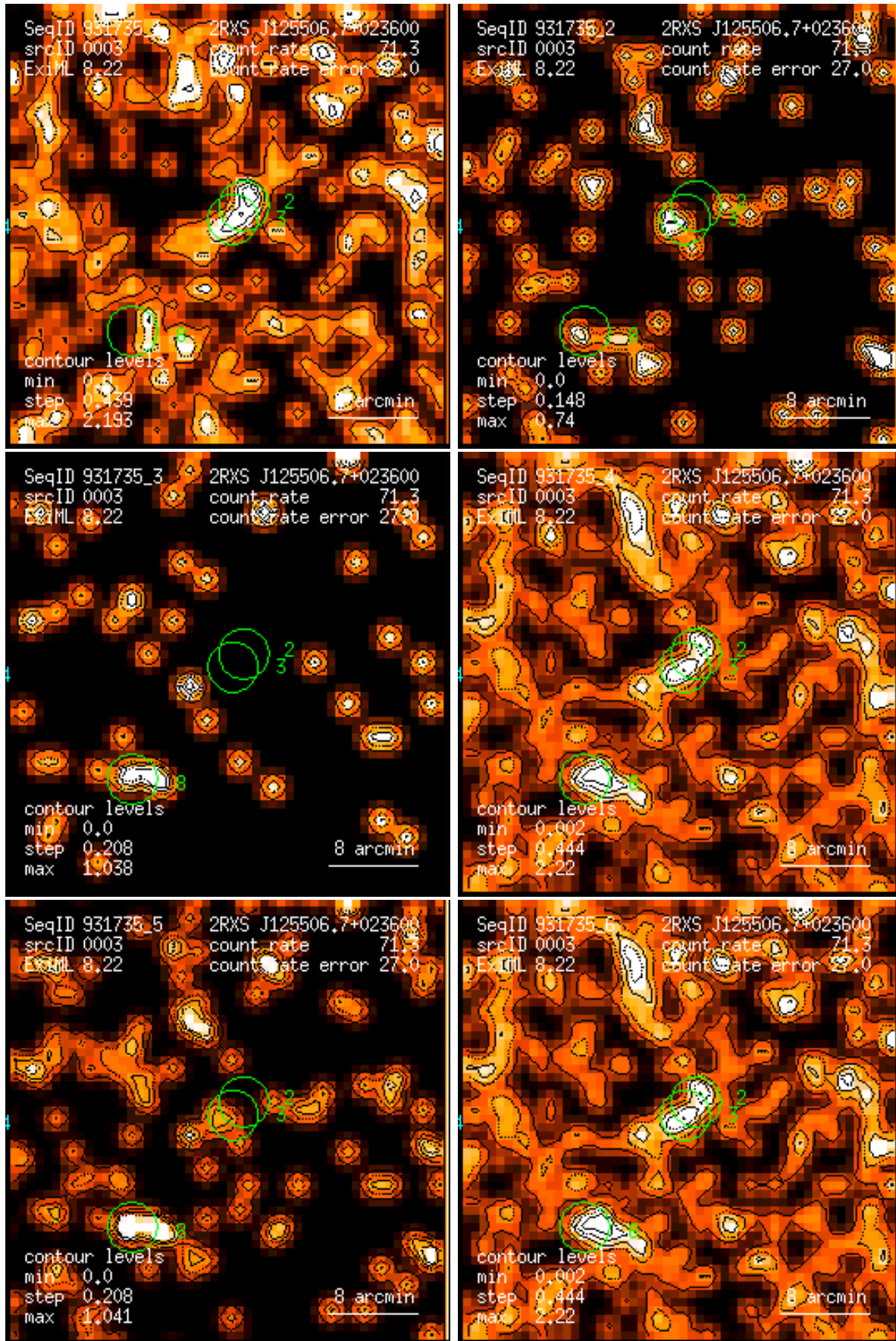
Figure 3: RASS 931735: detection 0003: band rate images, Gaussian filter: (1) PSPC channels 11 – 41, (2) 52 – 90, (3) 91 – 201, (4) 11 – 235, (5) 52 – 201, (6) 11 – 201. Broad band rates in counts/ks. Band rate contour levels in counts/ks/arcmin 2 .
