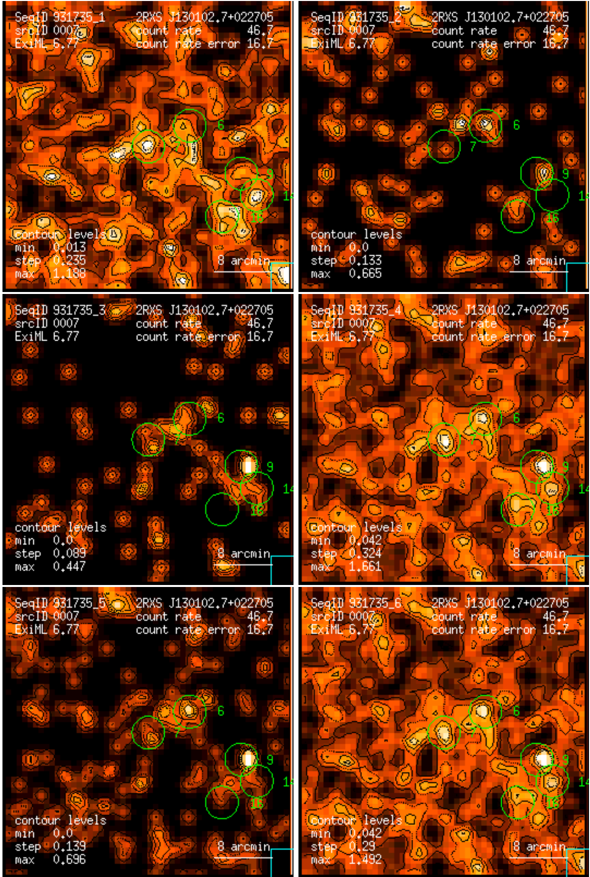
Figure 7: RASS 931735: detection 0007: band rate images, Gaussian filter: (1) PSPC channels 11 – 41, (2) 52 – 90, (3) 91 – 201, (4) 11 – 235, (5) 52 – 201, (6) 11 – 201. Broad band rates in counts/ks. Band rate contour levels in counts/ks/arcmin 2 .
