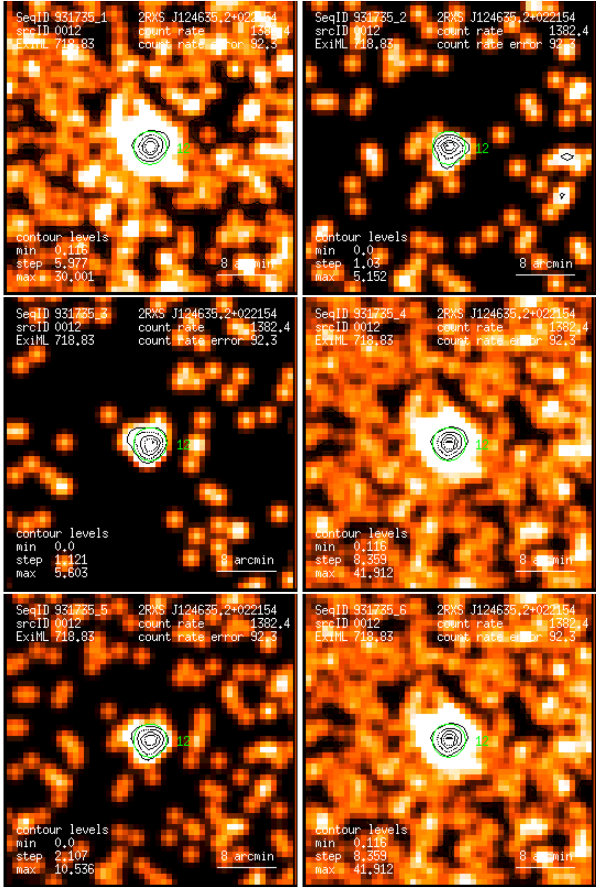
Figure 12: RASS 931735: detection 0012: band rate images, Gaussian filter: (1) PSPC channels 11 – 41, (2) 52 – 90, (3) 91 – 201, (4) 11 – 235, (5) 52 – 201, (6) 11 – 201. Broad band rates in counts/ks. Band rate contour levels in counts/ks/arcmin 2 .
