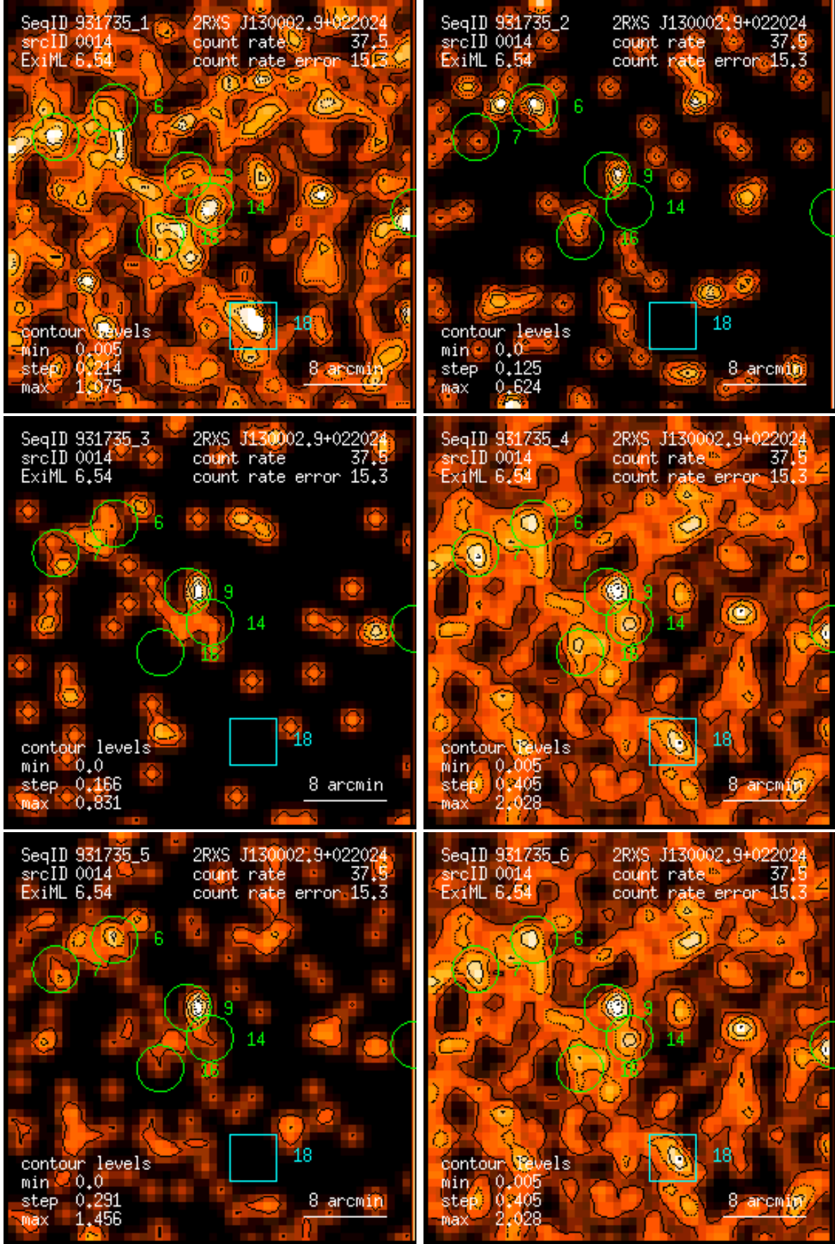
Figure 14: RASS 931735: detection 0014: band rate images, Gaussian filter: (1) PSPC channels 11 – 41, (2) 52 – 90, (3) 91 – 201, (4) 11 – 235, (5) 52 – 201, (6) 11 – 201. Broad band rates in counts/ks. Band rate contour levels in counts/ks/arcmin 2 .
