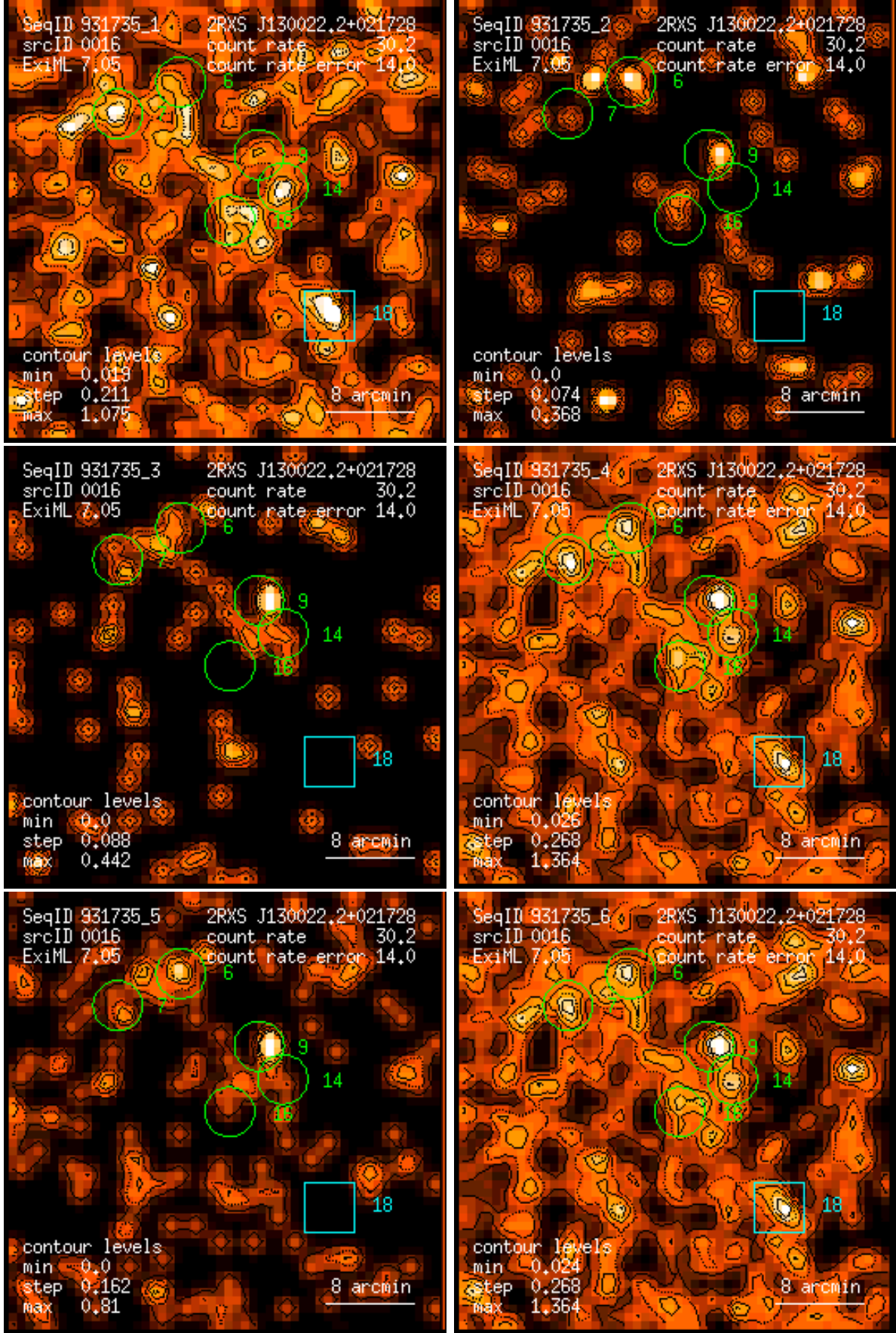
Figure 16: RASS 931735: detection 0016: band rate images, Gaussian filter: (1) PSPC channels 11 – 41, (2) 52 – 90, (3) 91 – 201, (4) 11 – 235, (5) 52 – 201, (6) 11 – 201. Broad band rates in counts/ks. Band rate contour levels in counts/ks/arcmin 2 .
