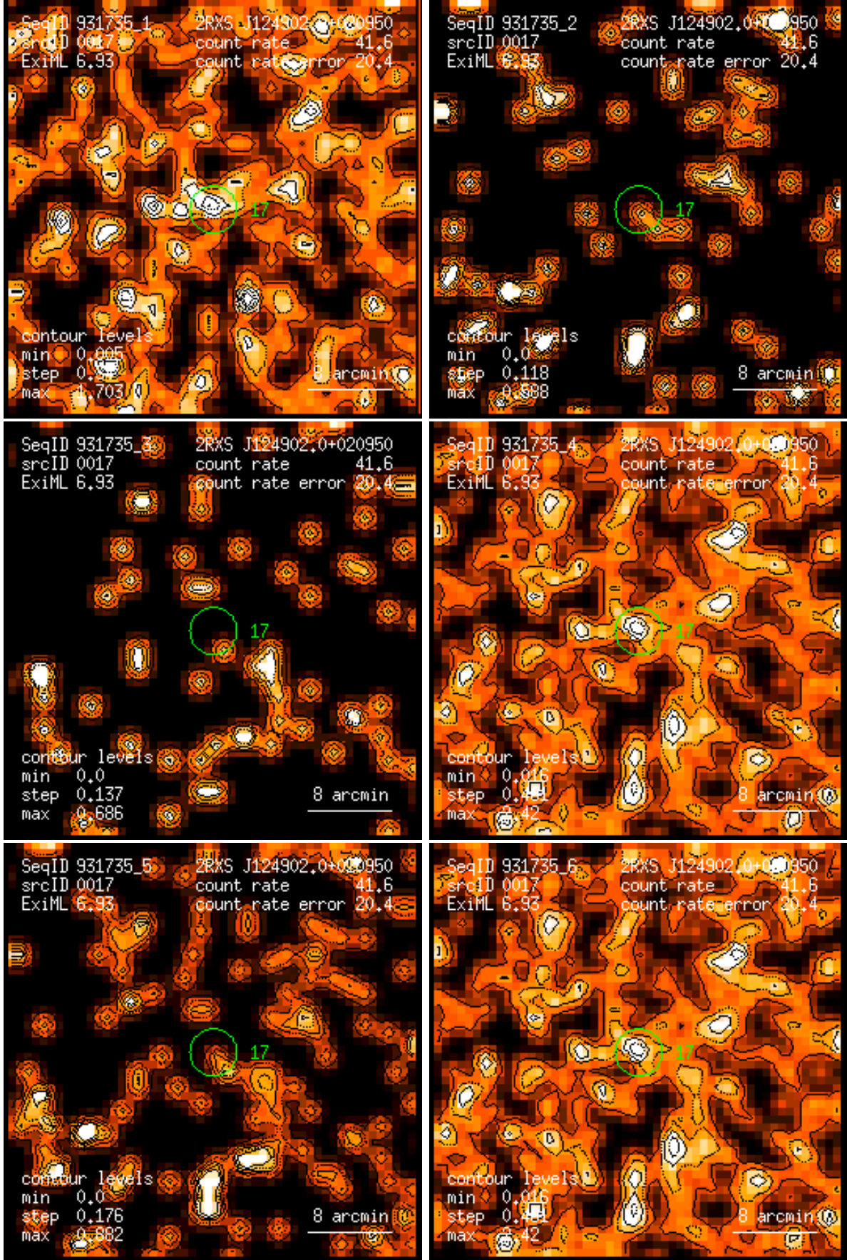
Figure 17: RASS 931735: detection 0017: band rate images, Gaussian filter: (1) PSPC channels 11 – 41, (2) 52 – 90, (3) 91 – 201, (4) 11 – 235, (5) 52 – 201, (6) 11 – 201. Broad band rates in counts/ks. Band rate contour levels in counts/ks/arcmin 2 .
