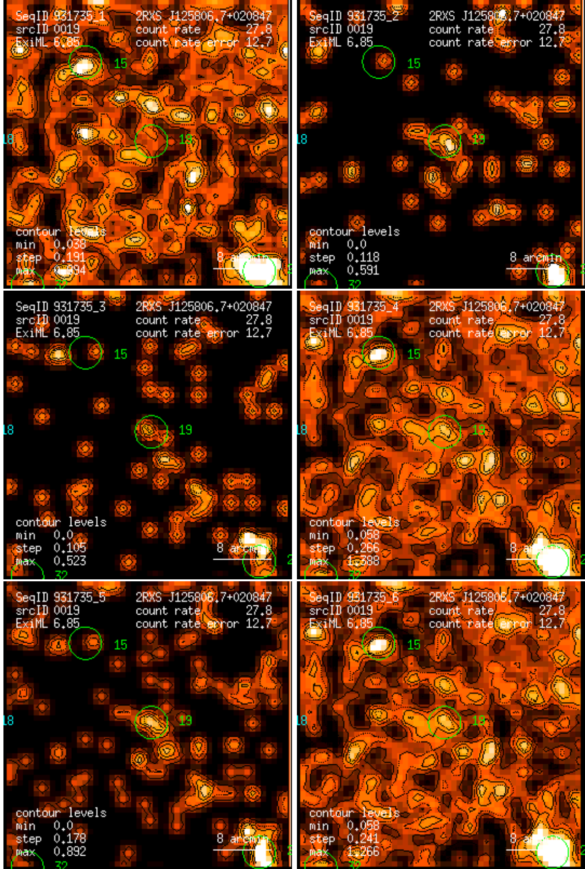
Figure 19: RASS 931735: detection 0019: band rate images, Gaussian filter: (1) PSPC channels 11 – 41, (2) 52 – 90, (3) 91 – 201, (4) 11 – 235, (5) 52 – 201, (6) 11 – 201. Broad band rates in counts/ks. Band rate contour levels in counts/ks/arcmin 2 .
