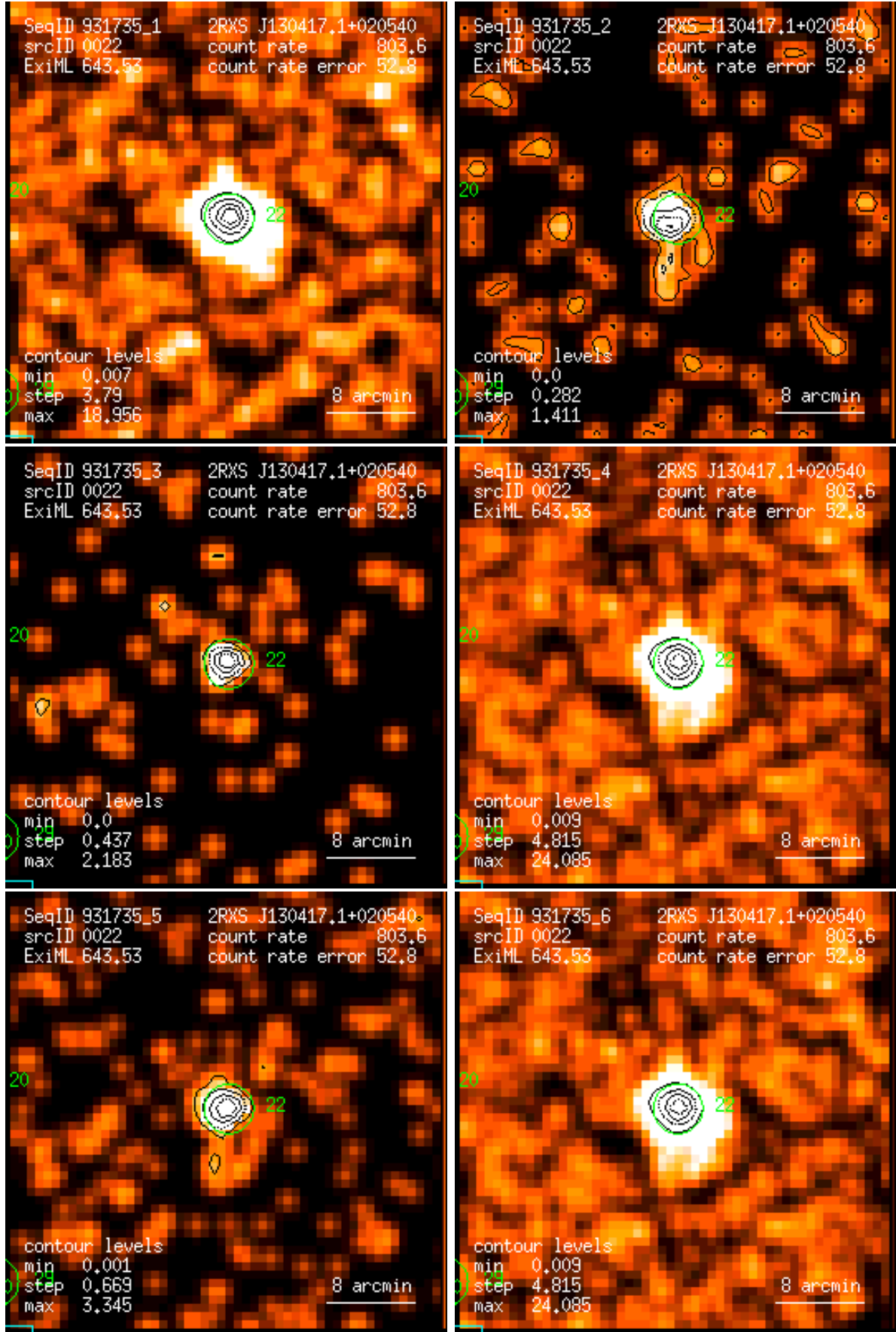
Figure 22: RASS 931735: detection 0022: band rate images, Gaussian filter: (1) PSPC channels 11 – 41, (2) 52 – 90, (3) 91 – 201, (4) 11 – 235, (5) 52 – 201, (6) 11 – 201. Broad band rates in counts/ks. Band rate contour levels in counts/ks/arcmin 2 .
