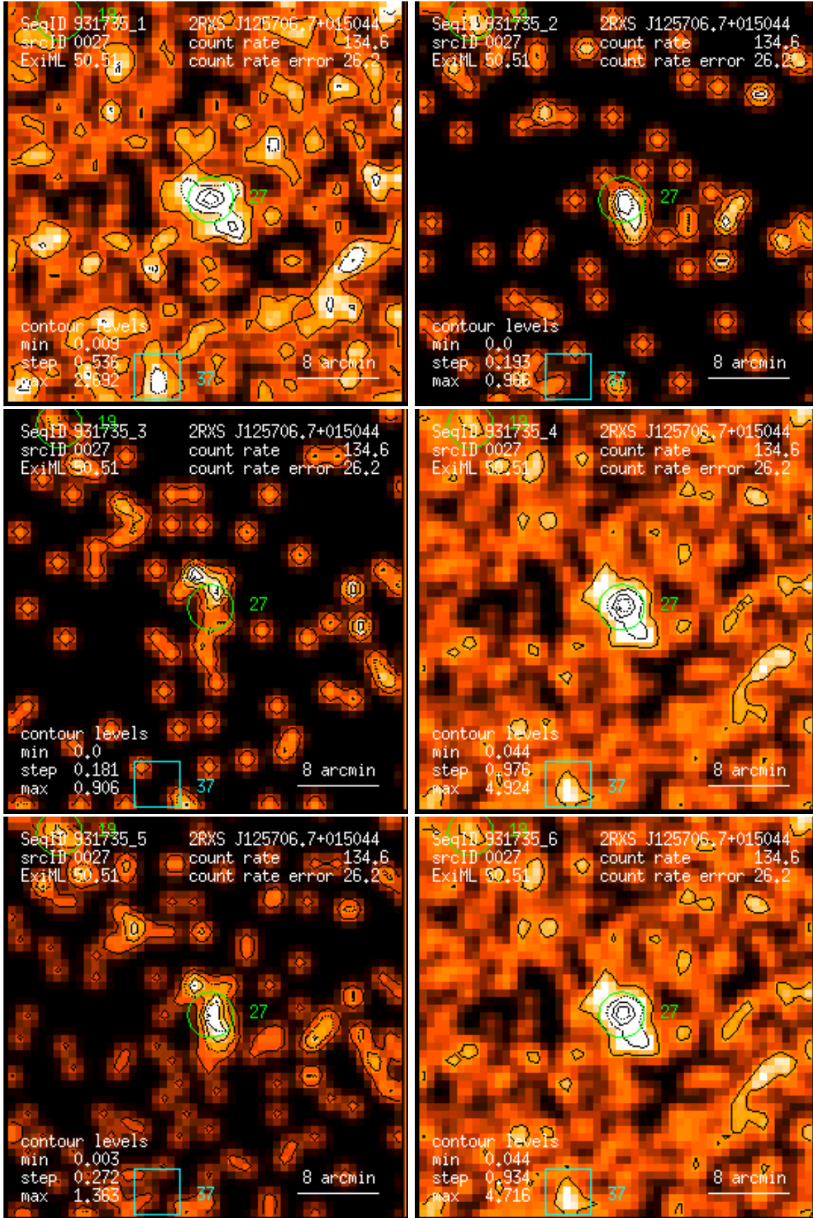
Figure 27: RASS 931735: detection 0027: band rate images, Gaussian filter: (1) PSPC channels 11 – 41, (2) 52 – 90, (3) 91 – 201, (4) 11 – 235, (5) 52 – 201, (6) 11 – 201. Broad band rates in counts/ks. Band rate contour levels in counts/ks/arcmin 2 .
