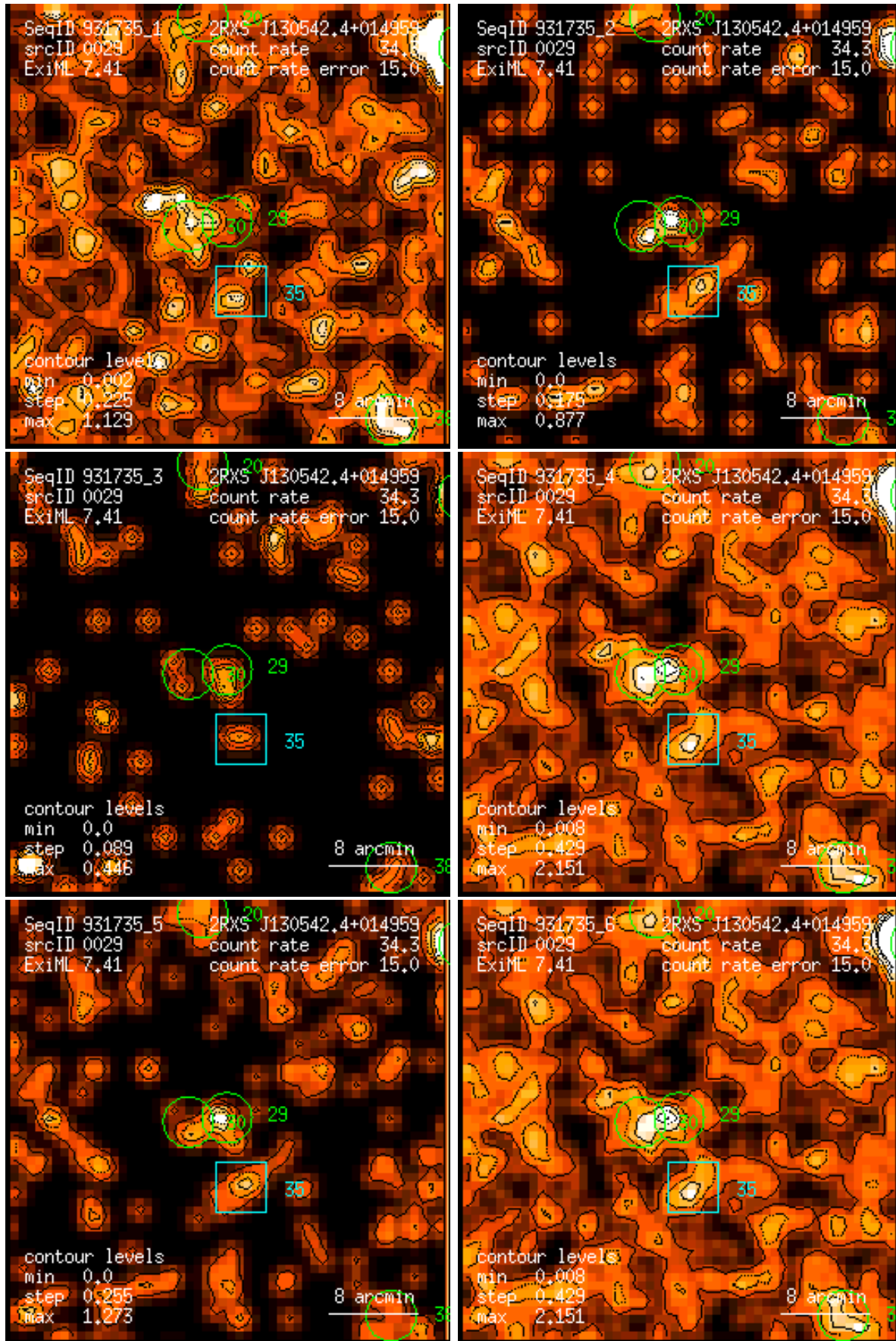
Figure 29: RASS 931735: detection 0029: band rate images, Gaussian filter: (1) PSPC channels 11 – 41, (2) 52 – 90, (3) 91 – 201, (4) 11 – 235, (5) 52 – 201, (6) 11 – 201. Broad band rates in counts/ks. Band rate contour levels in counts/ks/arcmin 2 .
