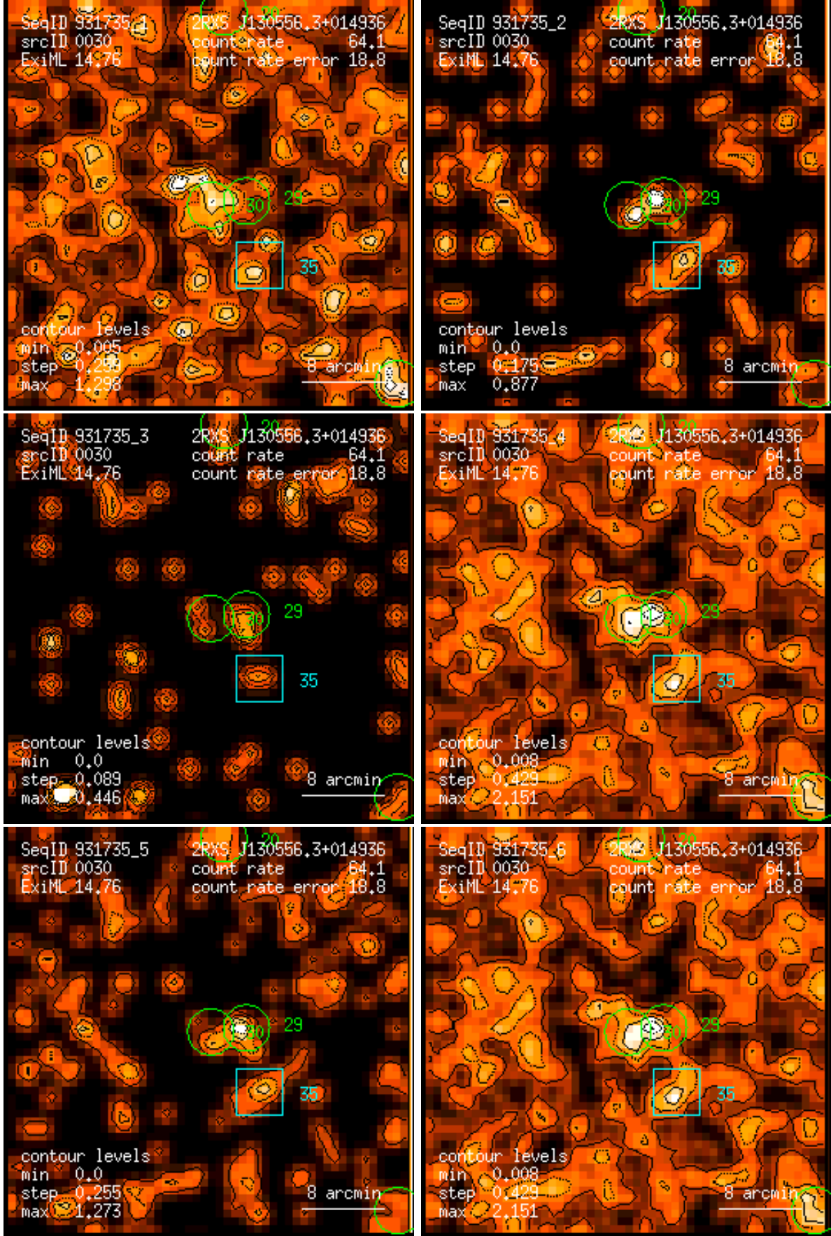
Figure 30: RASS 931735: detection 0030: band rate images, Gaussian filter: (1) PSPC channels 11 – 41, (2) 52 – 90, (3) 91 – 201, (4) 11 – 235, (5) 52 – 201, (6) 11 – 201. Broad band rates in counts/ks. Band rate contour levels in counts/ks/arcmin 2 .
