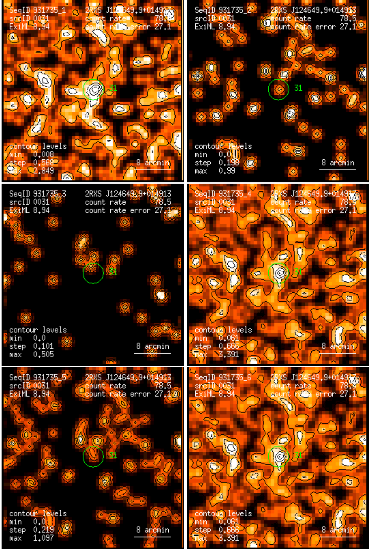
Figure 31: RASS 931735: detection 0031: band rate images, Gaussian filter: (1) PSPC channels 11 – 41, (2) 52 – 90, (3) 91 – 201, (4) 11 – 235, (5) 52 – 201, (6) 11 – 201. Broad band rates in counts/ks. Band rate contour levels in counts/ks/arcmin 2 .
