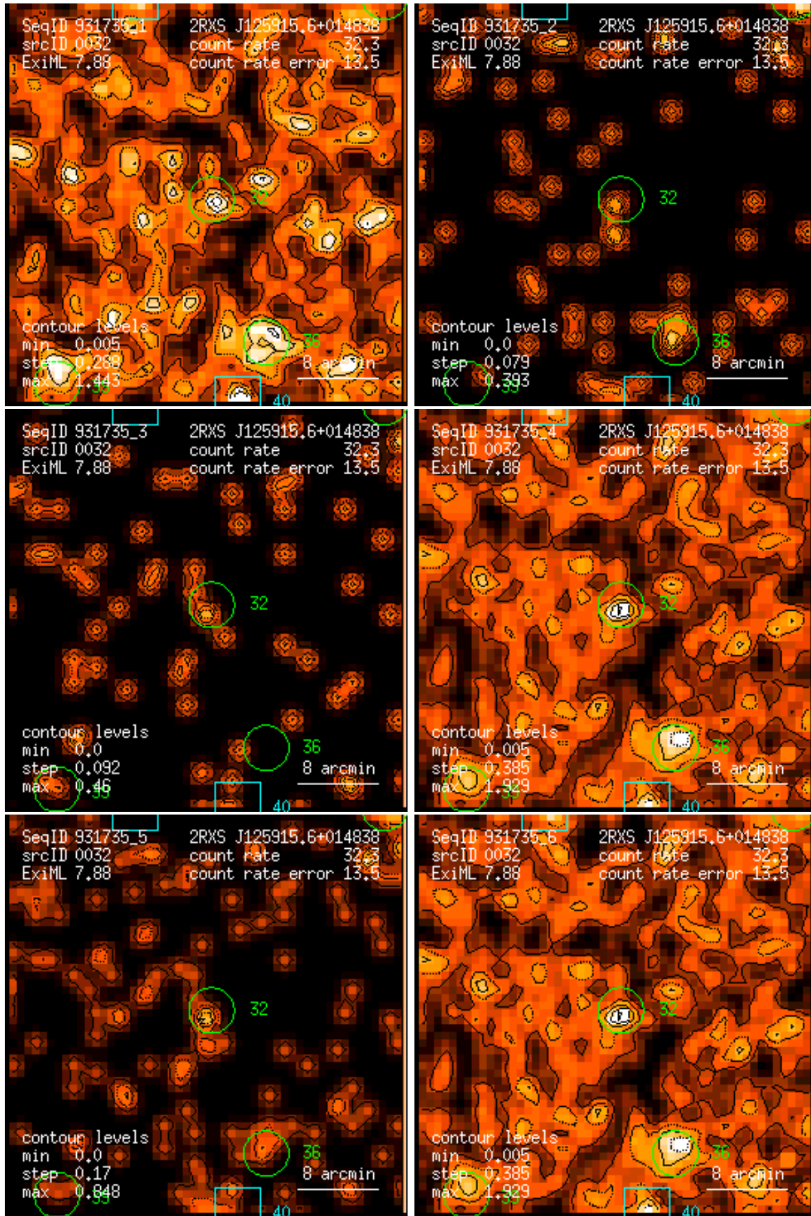
Figure 32: RASS 931735: detection 0032: band rate images, Gaussian filter: (1) PSPC channels 11 – 41, (2) 52 – 90, (3) 91 – 201, (4) 11 – 235, (5) 52 – 201, (6) 11 – 201. Broad band rates in counts/ks. Band rate contour levels in counts/ks/arcmin 2 .
