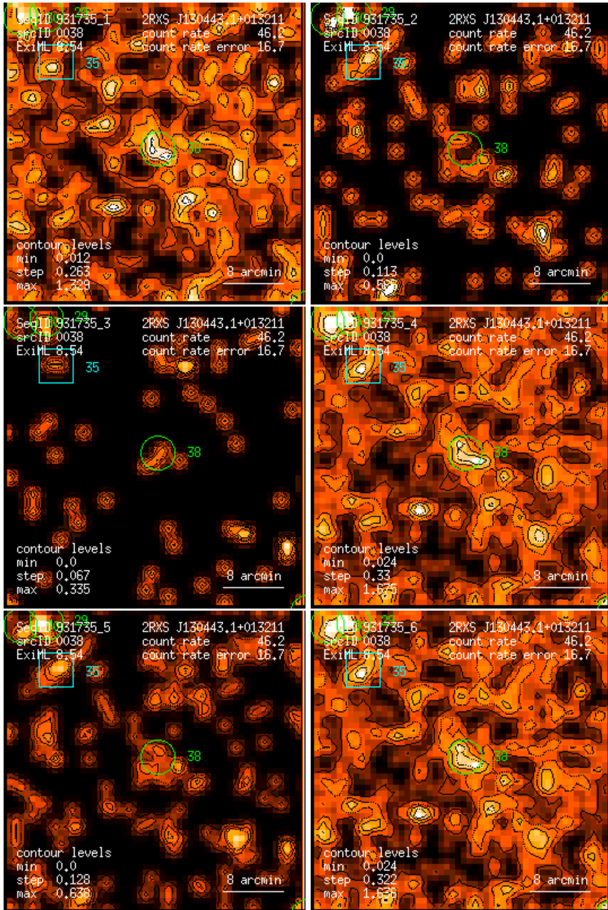
Figure 38: RASS 931735: detection 0038: band rate images, Gaussian filter: (1) PSPC channels 11 – 41, (2) 52 – 90, (3) 91 – 201, (4) 11 – 235, (5) 52 – 201, (6) 11 – 201. Broad band rates in counts/ks. Band rate contour levels in counts/ks/arcmin 2 .
